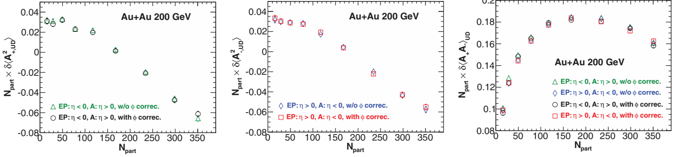
FIG. 21. (Color online) The statistical and detector effect subtracted asymmetry correlations, \delta\langle A_{\pm, \text{LR}}^2 \rangle (left panel), \delta\langle A_{\pm, \text{LR}}^2 \rangle (middle panel), and \delta\langle A_+ A_- \rangle_{\text{LR}} (right panel), multiplied by the number of participants N_{\text{part}} before and after the corrections for the \phi -dependent acceptance \times efficiency. This figure corresponds to Fig. 18. The error bars are statistical only.
