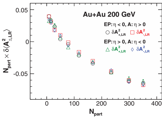
FIG. 22. (Color online) Dynamical charge asymmetry variance after removing the statistical and detector effects, \delta\langle A_{\pm, \text{LR}}^2 \rangle = \langle A_{\pm, \text{LR}}^2 \rangle - \langle A_{\pm, \text{LR}, \text{stat+det}}^2 \rangle , scaled by the number of participants N_{\text{part}} . The results are consistent between positive and negative \eta regions and between positive and negative charges. Error bars are statistical only.
