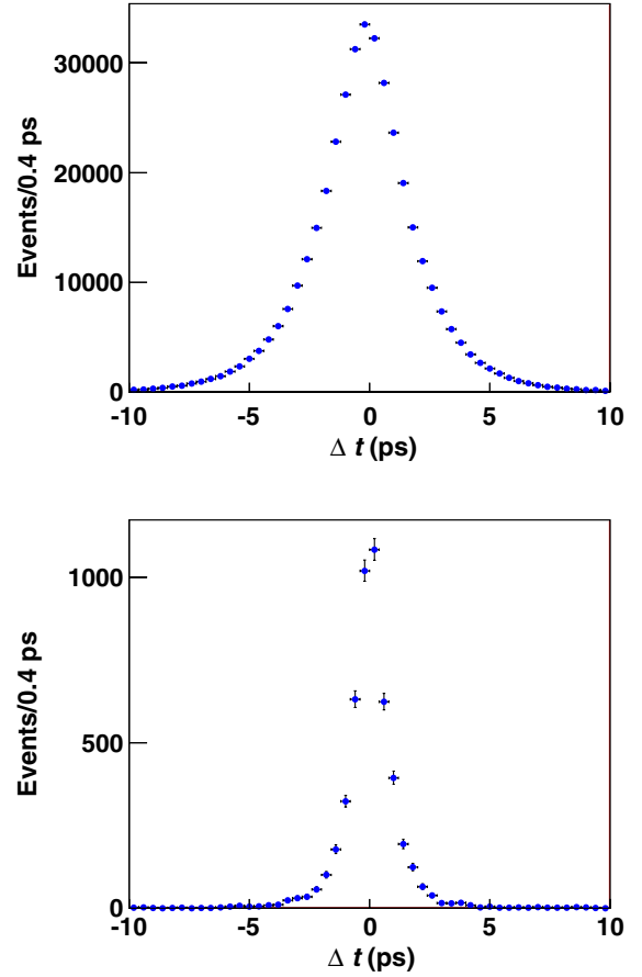
FIG. 4 (color online). Distribution of \Delta t in simulated B^0 \rightarrow \rho^+ \pi^+ signal events (top) and in off-resonance data (bottom).
