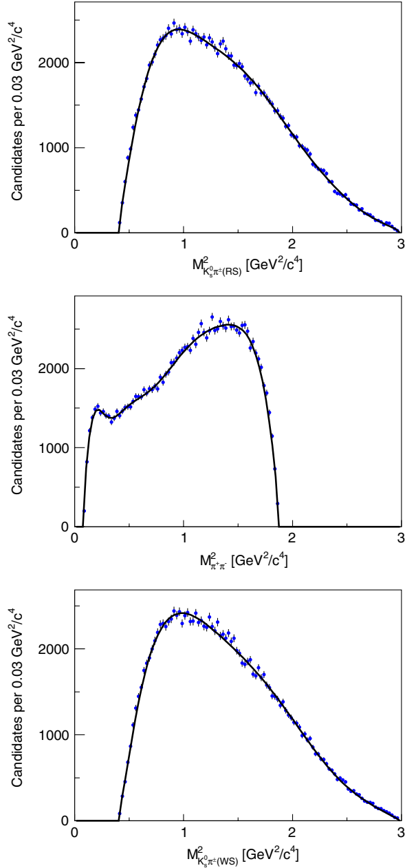
FIG. 3 (color online). Squared invariant-mass distributions of the simulated events used for the determination of the relative reconstruction efficiency over the Dalitz plot, together with the corresponding fit projections.
