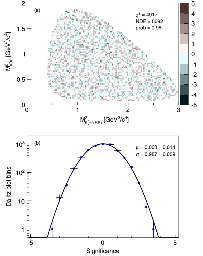
FIG. 6 (color online). Distribution of the asymmetry significance (a) as a function of the squared K_S^0 \pi^+ \pi^- masses and (b) as a histogram.
