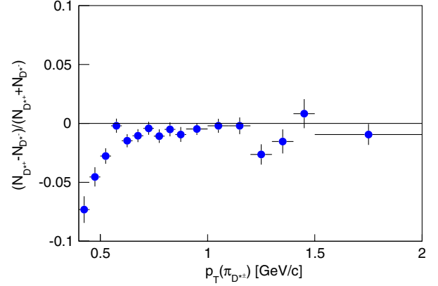
FIG. 5 (color online). Asymmetry between the numbers of reconstructed D^{*+} and D^{*-} candidates as a function of the soft pion's p_T .
