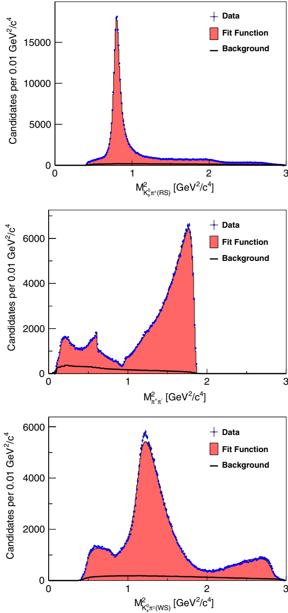
FIG. 4 (color online). Projections of the Dalitz-plot fit on the individual two-body masses, together with the corresponding distributions in data.
