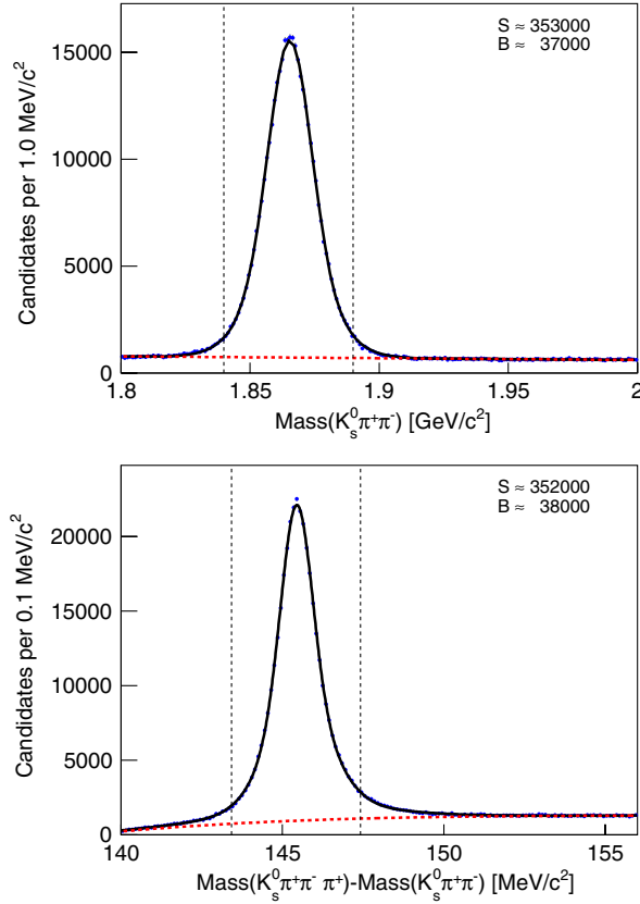
FIG. 1 (color online). The M(K_S^0 \pi^+ \pi^-) and \Delta M data distributions (points with error bars) with fit results overlaid. The dashed lines correspond to the background contributions. The vertical lines indicate signal ranges used for further analysis. The M(K_S^0 \pi^+ \pi^-) ( \Delta M ) distribution contains only candidates populating the signal \Delta M [ M(K_S^0 \pi^+ \pi^-) ] range.
