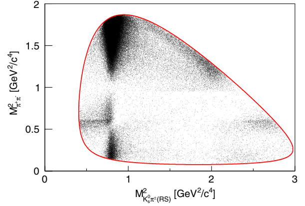
FIG. 2 (color online). Dalitz plot of the decay D^0/\bar{D}^0 \rightarrow K_S^0 \pi^+ \pi^- , where the squared invariant masses of the two-body combinations K_S^0 \pi^\pm (RS) and \pi^+ \pi^- are chosen as kinematic quantities. The solid line indicates the kinematic boundaries.
