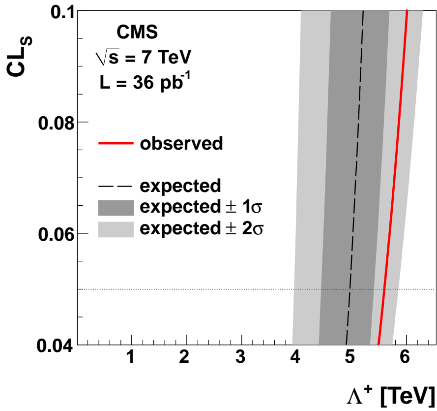
Figure 2: Observed CL_s (solid line) and expected CL_s (dashed line) with one (two) standard deviation(s) indicated by the dark (light) band as a function of the contact interaction scale \Lambda^+ . The 95% confidence level limits on \Lambda^+ are extracted from the intersections of the observed and expected CL_s lines with the horizontal line at CL_s=0.05 .
