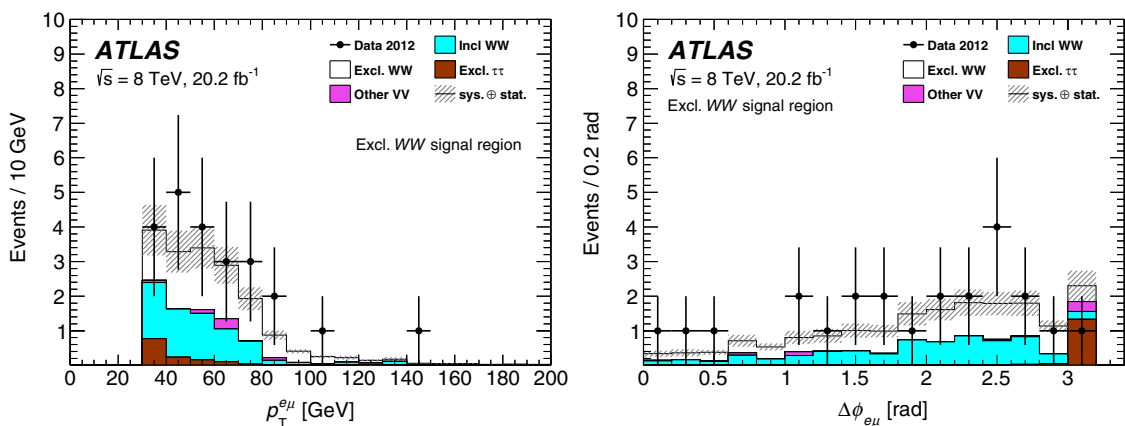
FIG. 12. The p_T^{e\mu} (left) and \Delta\phi_{e\mu} (right) distributions in the exclusive W^+W^- signal region. The inclusive W^+W^- estimate includes small contributions from other backgrounds (Drell-Yan, W + jets, and top-quark production).
