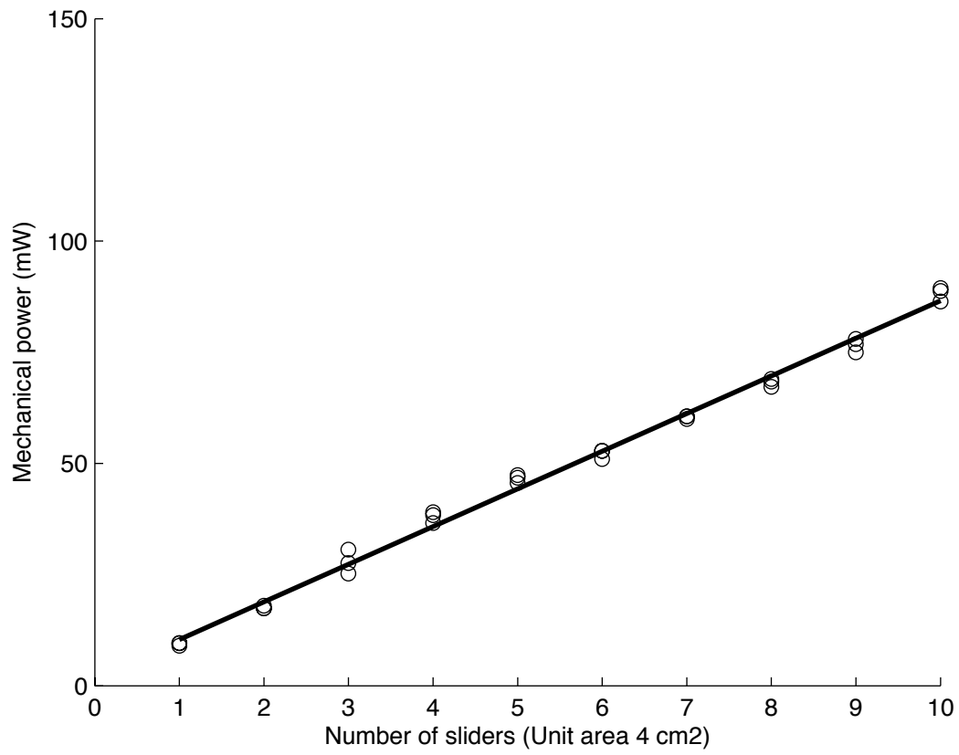
Figure 4: Experiment 1: Mechanical power versus number of sliders. Plate 200x300x2mm, high damping ( T_r=0.4s ), thick sliders 20x20x20mm, low roughness R_a=1\mu m . \circ , measurement; —, linear regression.
