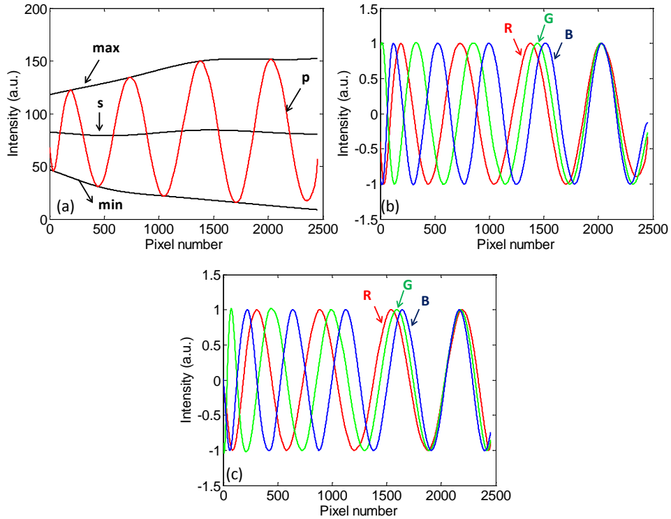
Fig. 1. Eliminating the non-uniform signal bias using min-max method: (a) The original signal- p , envelopes of maxima and minima and the mean 's', (b) R, G, B components after removing non uniform bias, and (c) HT generated signals corresponding to the signals in Fig. 1(b).
