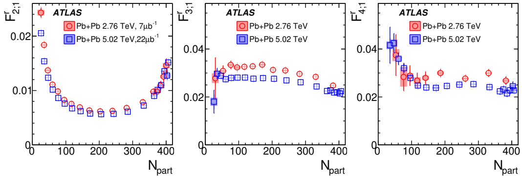
Figure 11: Centrality dependence of F_{2;1}^r (left panel), F_{3;1}^r (middle panel) and F_{4;1}^r (right panel) for Pb+Pb at 2.76 TeV (circles) and 5.02 TeV (squares). The error bars and shaded boxes are statistical and systematic uncertainties, respectively. The widths of the centrality intervals are not fixed but are optimised to reduce the uncertainty.
