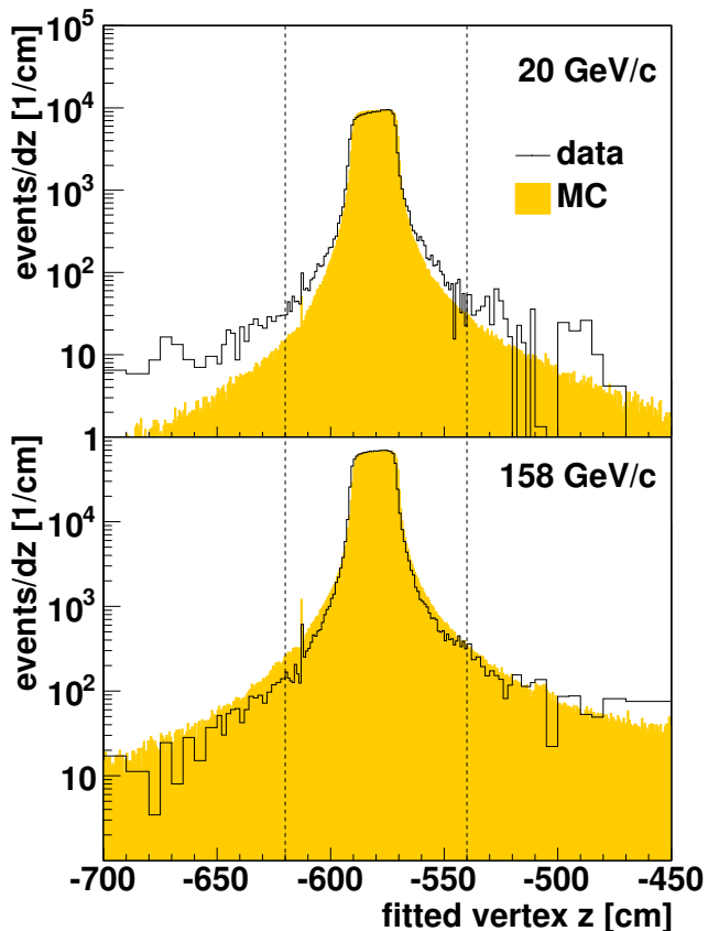
Fig. 8: (Colour online) Distribution of fitted vertex z coordinate for p+p interactions at 20 ( top ) and 158 GeV/c ( bottom ). The black line shows the data after target removed subtraction (see Sec. 5.4). The filled area shows the distribution for the reconstructed Monte Carlo simulation. This distribution was normalised to the total integral of the data plot. The dashed vertical lines show the z vertex selection range.
