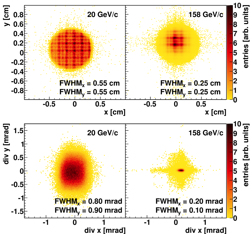
Fig. 2: (Colour online) Top : The beam spot as measured by BPD-3 after the \sqrt{|V|} cut described in the text for 20 GeV/c ( left ) and 158 GeV/c ( right ) beams. Bottom : The beam divergence in x and y for 20 GeV/c ( left ) and 158 GeV/c ( right ) beams. All distributions were arbitrarily scaled to the full colour scale. Widths of the distributions are given in the legend.
