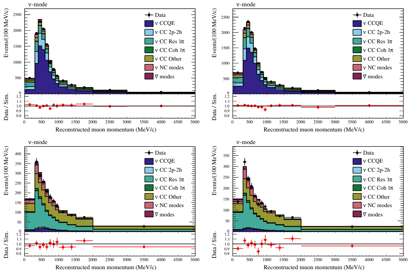
FIG. 14. Data MC comparison of \nu -mode \nu_\mu CC- 0\pi (top) and CC- 1\pi^+ (bottom) samples in FGD1 (left) and FGD2 (right) after the ND280 fit. The simulation is broken down by neutrino reaction type.
