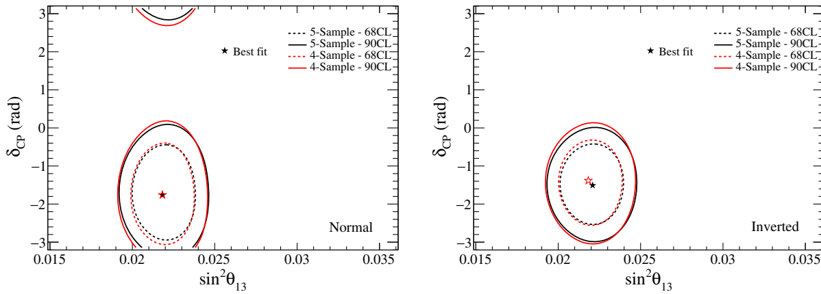
FIG. 42. A comparison of two-dimensional constant \Delta\chi^2 contours in the \delta_{CP} - \sin^2\theta_{13} plane using T2K data with the reactor constraint, for both four-sample (red) and five-sample (black) analyses with normal (left) and inverted (right) mass ordering hypotheses. The contours are produced by marginalizing the likelihood with respect to all parameters other than the parameters of interest.
