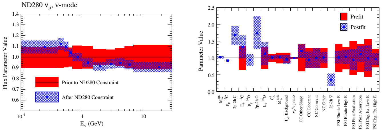
FIG. 31. The nominal values (red) and postfit values (blue) of the ND 280 \nu -mode \nu_\mu flux (left) and the cross section (right) parameters, shown as a fraction of their nominal value, following the near detector fit to the alternative 2p2h ND280 simulated data.
