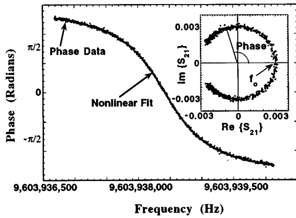
FIG. 4. Measured phase as a function of frequency for measured data (SNR ≈ 31), both data and fit are shown. Inset is the translated and rotated circle, where its center is at the origin and the phase to each point is calculated from the positive real axis.
