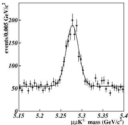
FIG. 4. The mass distribution of the J/\psi K^\pm candidates both with and without SVX information. The curve is a Gaussian signal plus linear background from the likelihood fit.
