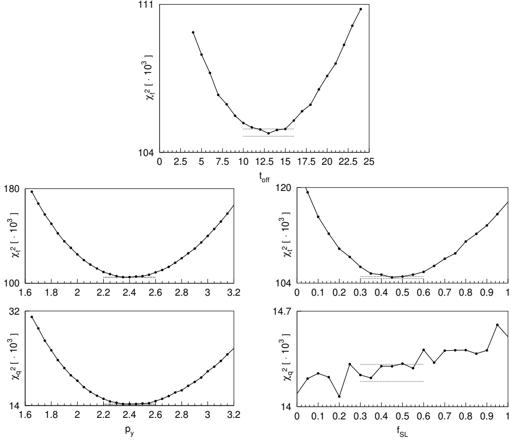
Figure 13: Behavior of \chi^2 and \chi^2_q in the vicinity of the fit minimum vs. t_{\text{off}} , p_y , and f_{\text{SL}} . All plots are shown on a linear scale. Horizontal dotted lines show the \pm 1\sigma range due to purely statistical fluctuations in the simulation estimated for the best-fit model. The minimum in t_{\text{off}} and f_{\text{SL}} is a feature of \chi^2 but not \chi^2_q .
