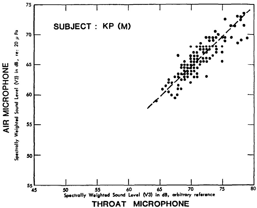
FIGURE 13. OBSERVED RELATIONSHIP BETWEEN CONVENTIONAL AIR MICROPHONE AND THROAT MICROPHONE
