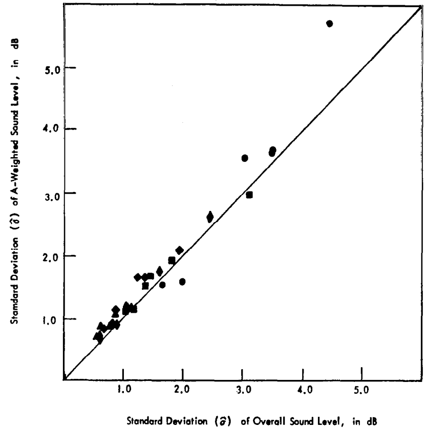
FIGURE 3. COMPARISON OF MEANS AND STANDARD DEVIATIONS BETWEEN A-WEIGHTED AND OVERALL SOUND LEVELS
