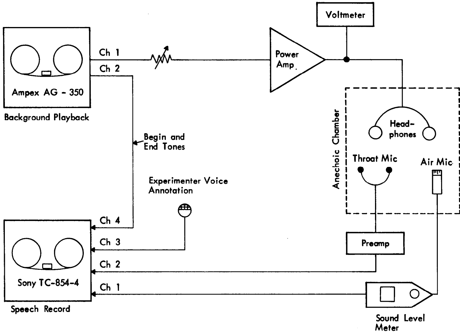
FIGURE B-2. BLOCK DIAGRAM OF BACKGROUND NOISE GENERATION AND SPEECH RECORDING INSTRUMENTATION
