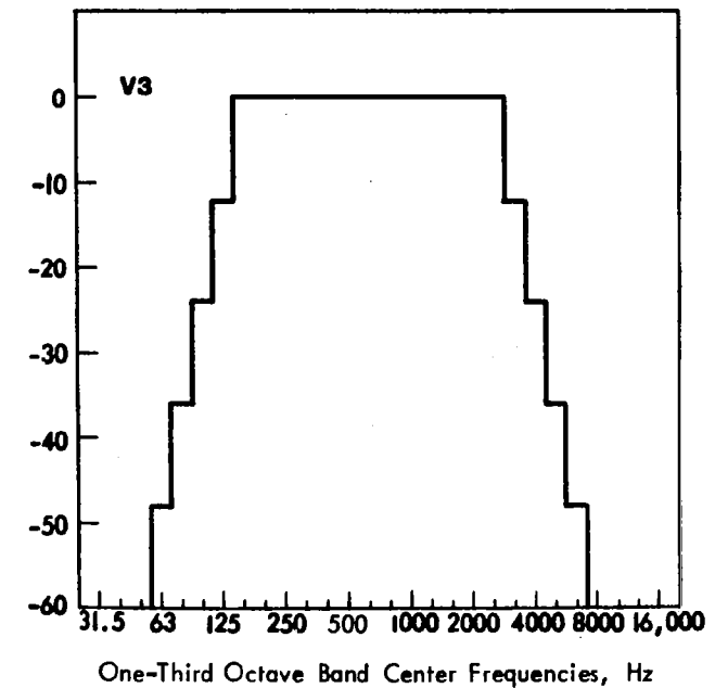
FIGURE 2. ONE-THIRD OCTAVE BAND FREQUENCY WEIGHTINGS FOR VARIOUS SPEECH LEVEL MEASURES
