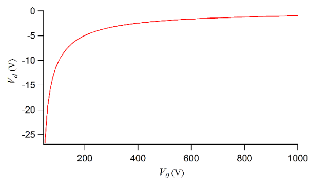
Figure 1. Simulation of the effect of bias voltage on the measured EFB voltage change for differential weighing of a 100 \mu\text{g} mass.
