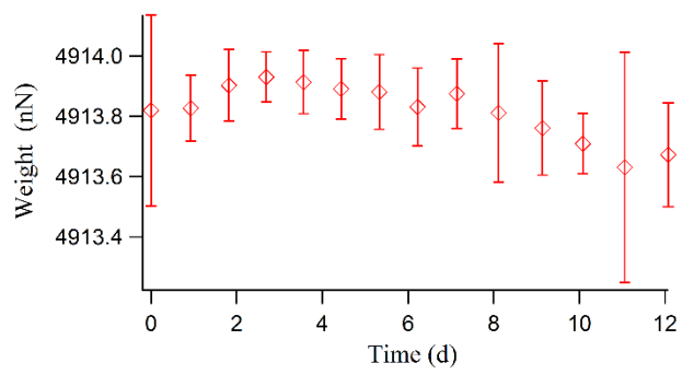
Fig. 3. Weight of a 500 \mu\text{g} mass artifact measured with the EFB. Error bars represent statistical uncertainty at k=2 , determined from the standard deviation of the mean in the same fashion as [8], but doubled to accommodate the coverage factor of 2.
