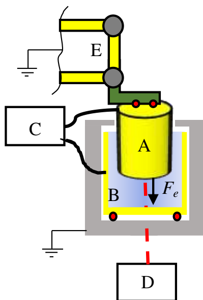
Fig. 2. Schematic diagram of the EFB. Inner capacitor cylinder (A) and outer capacitor cylinder (B) are connected to capacitance bridge (C) with coaxial cable (note, a relay network permits switching between the capacitance bridge and voltage amplifier, electrical connections denoted by solid curved lines). Laser interferometer (D) monitors the displacement of the inner cylinder guided by the balance mechanism (E), laser denoted by dashed line.
