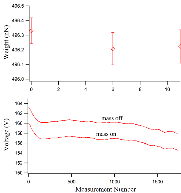
Fig. 4 Weight of a 50 \mu\text{g} mass measured with the EFB (top). Error bars represent statistical uncertainty at k=2 , as described in the caption of Fig. 3. The voltage measurements used to determine the third weight in the top graph. Only the positive polarity data are shown.
