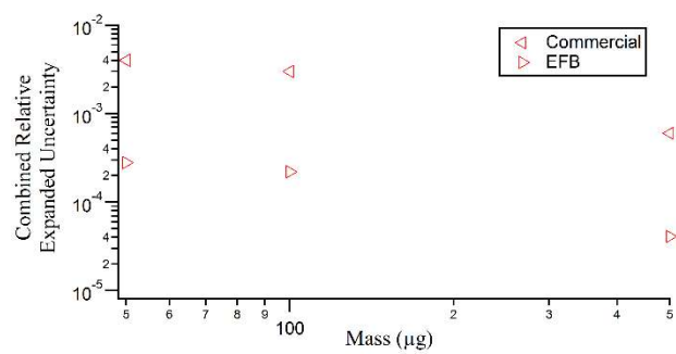
Fig. 5. Combined relative expanded uncertainty in submilligram mass calibration for submilligram masses. Data shown are the EFB calibrations shown in the current study and documented uncertainties from an accredited submilligram mass calibration facility.
