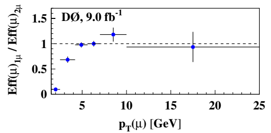
FIG. 9 (color online). The ratio of \pi \rightarrow \mu detection efficiencies for the inclusive-muon and dimuon data as a function of the muon transverse momentum. The horizontal dashed line shows the mean value for p_T(K) > 4.2 GeV.
