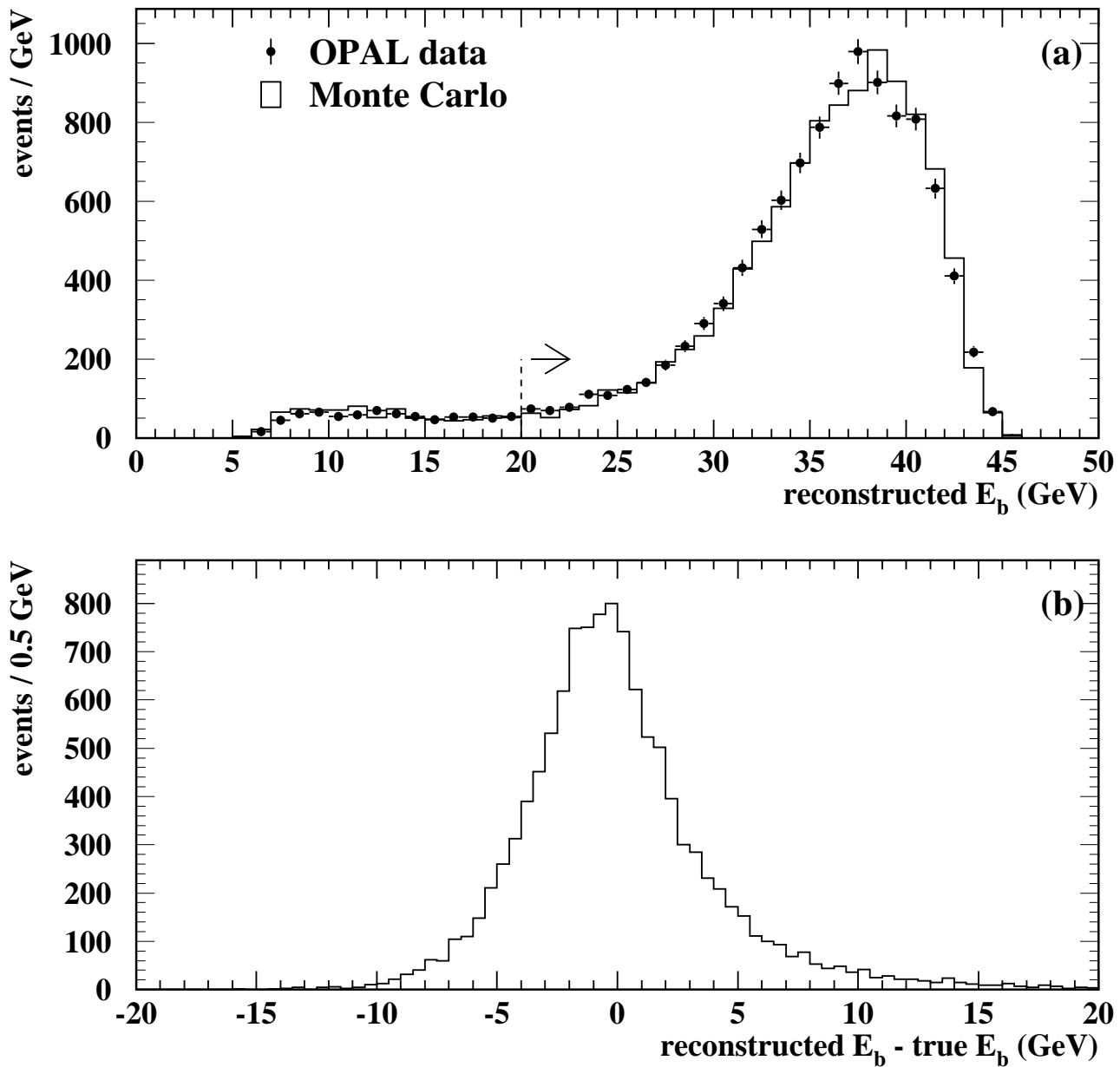
Figure 4: (a) Reconstructed b hadron energy distributions for data (points with error bars) and Monte Carlo (histogram). The position of the minimum energy cut is shown by the arrow. (b) Resolution of the reconstructed b hadron energy in Monte Carlo b\bar{b} events, after the minimum energy cut has been applied.
