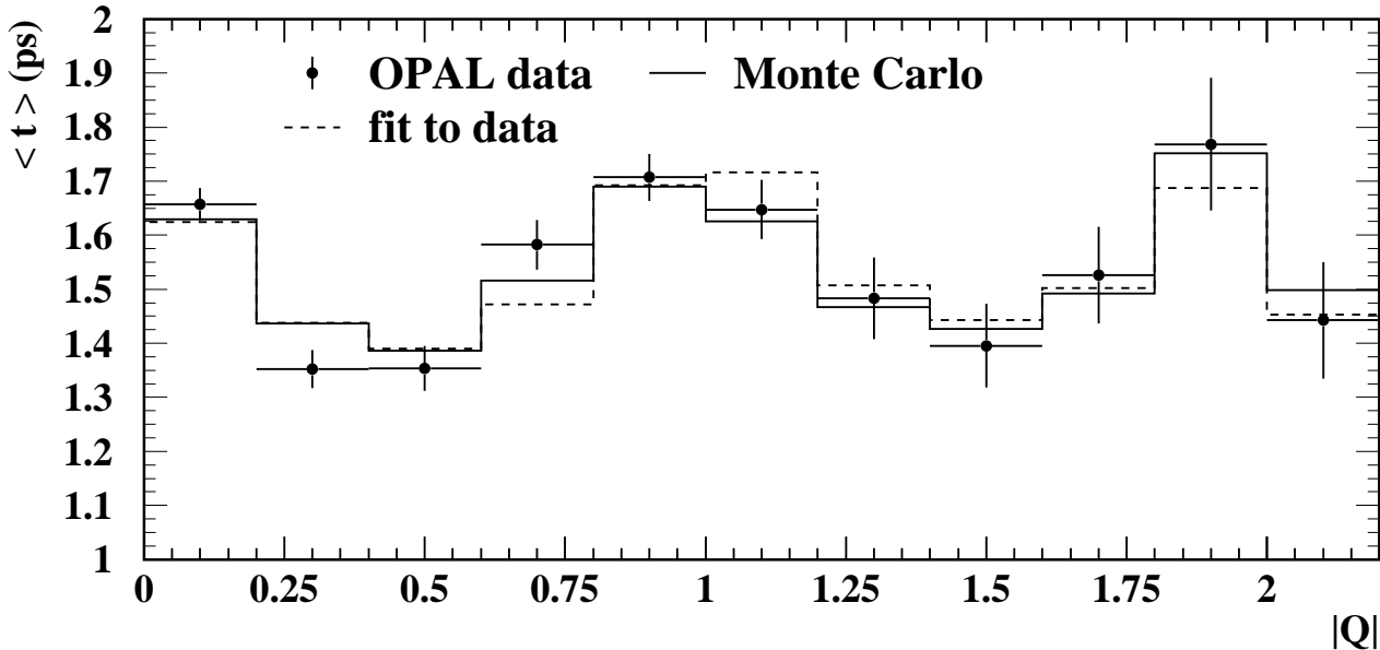
Figure 5: The distribution of mean excess decay time \langle t \rangle as a function of the modulus of the vertex charge |Q| . The data are shown by the points with error bars, and the Monte Carlo (reweighted to the same B^+ and B^0 lifetimes as measured in the data) distribution is shown by the solid line. The prediction of the fit is shown by the dashed line. The bin between |Q| = 2 and |Q| = 2.2 contains all events with |Q| > 2 .
