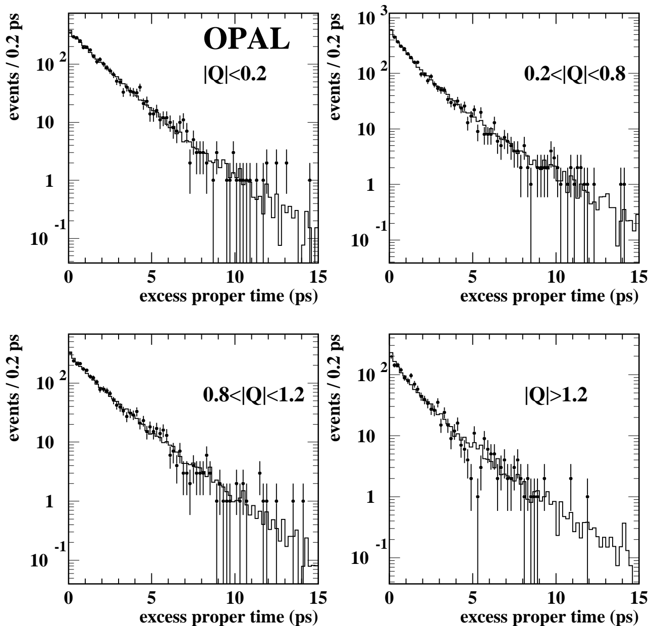
Figure 7: Distributions of excess proper time in four regions of absolute vertex charge |Q| , for data (points with error bars) and Monte Carlo simulation (histogram). The Monte Carlo B^+ and B^0 lifetimes have been reweighted to the same values as measured in the data.
