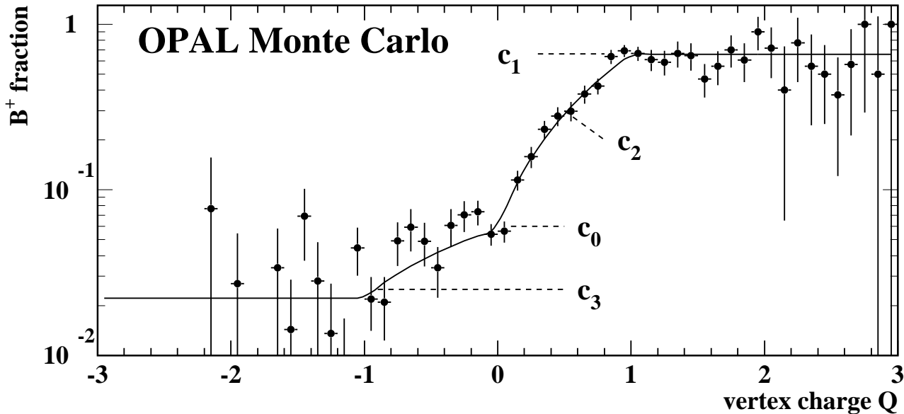
Figure 6: Fraction of B^+ vertices as a function of vertex charge Q in Monte Carlo b\bar{b} events (points with error bars). The parameterisation is shown by the solid line, and the levels c_0 , c_1 and c_3 by the dotted lines. The quadratic coefficient c_2 is used between Q = 0 and Q = 1 . Note that the non- b\bar{b} background fraction is not included, and the B^+ fraction is plotted using a logarithmic scale.
