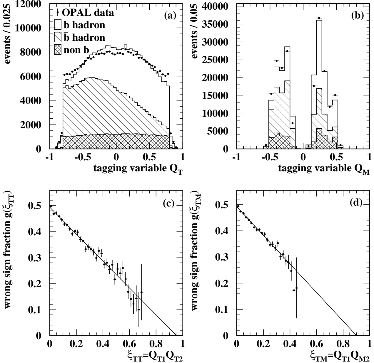
Figure 1: Production flavour tagging of b\bar{b} events: (a) Distribution of the flavour tagging variable Q_T in data (points) and Monte Carlo (histogram) T-tagged hemispheres. The contributions from b hadrons, \bar{b} hadrons and non-b backgrounds are shown. (b) The analogous distributions for the M-tag hemispheres. The 30% of the sample (90000 events in data) with Q_M = 0 are not shown. In both (a) and (b), the error bars on the data points are smaller than the symbols. (c) Distribution of the wrong sign fraction g(\xi_{TT}) in data double T-tagged events, with a linear fit superimposed. (d) Distribution of the wrong sign fraction g(\xi_{TM}) in data double T-tagged events, again with a linear fit superimposed.
