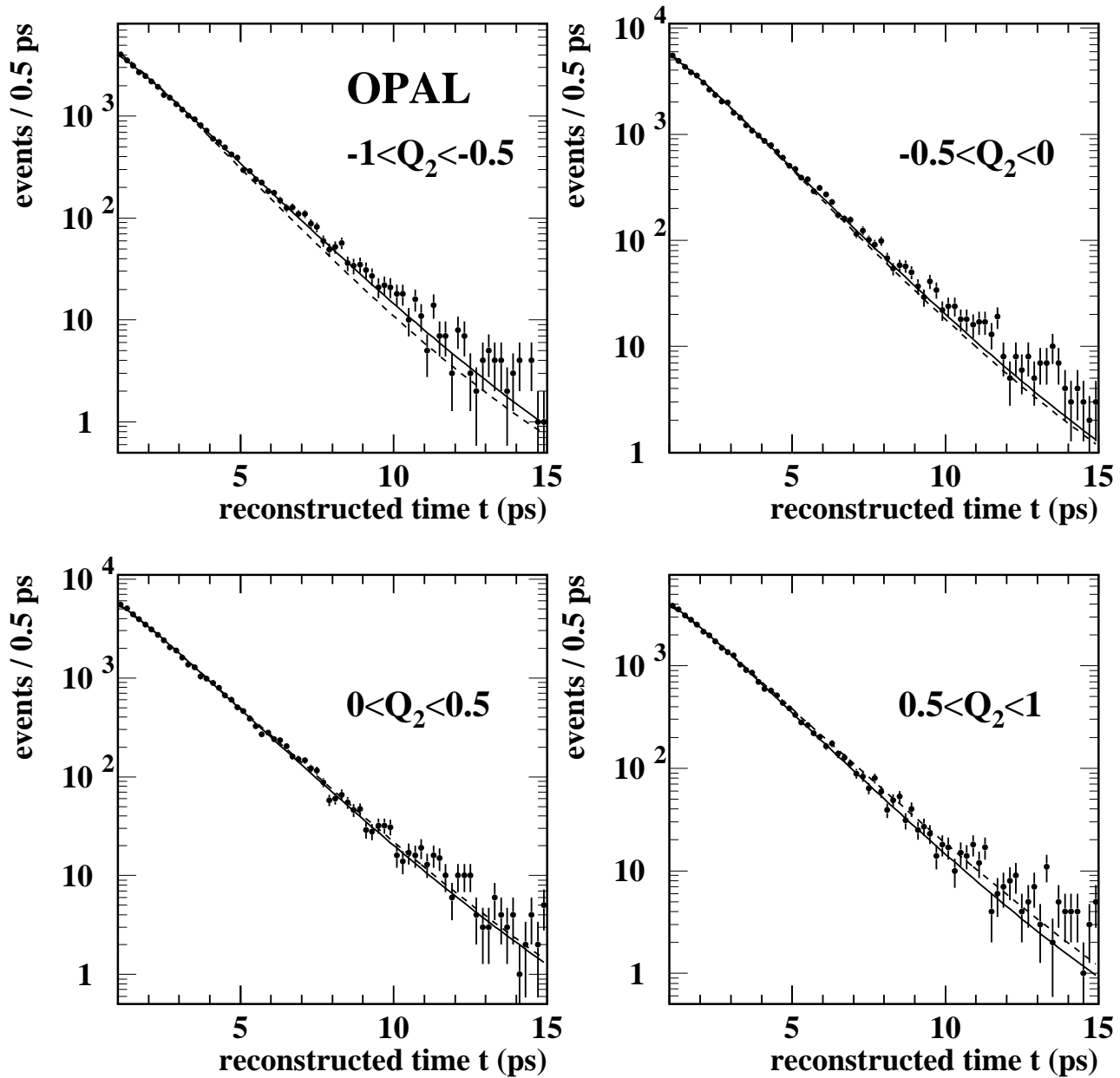
Figure 9: Distributions of reconstructed proper time t ( 1 < t < 15 ps) in four bins of tag variable Q_2 . The data are shown by the points with error bars, and the prediction of the fit by the solid lines. The expected distributions for a 20% difference between b and \bar{b} hadron lifetimes ( (\Delta\tau/\tau)_b = 0.2 ) are shown by the dotted lines.
