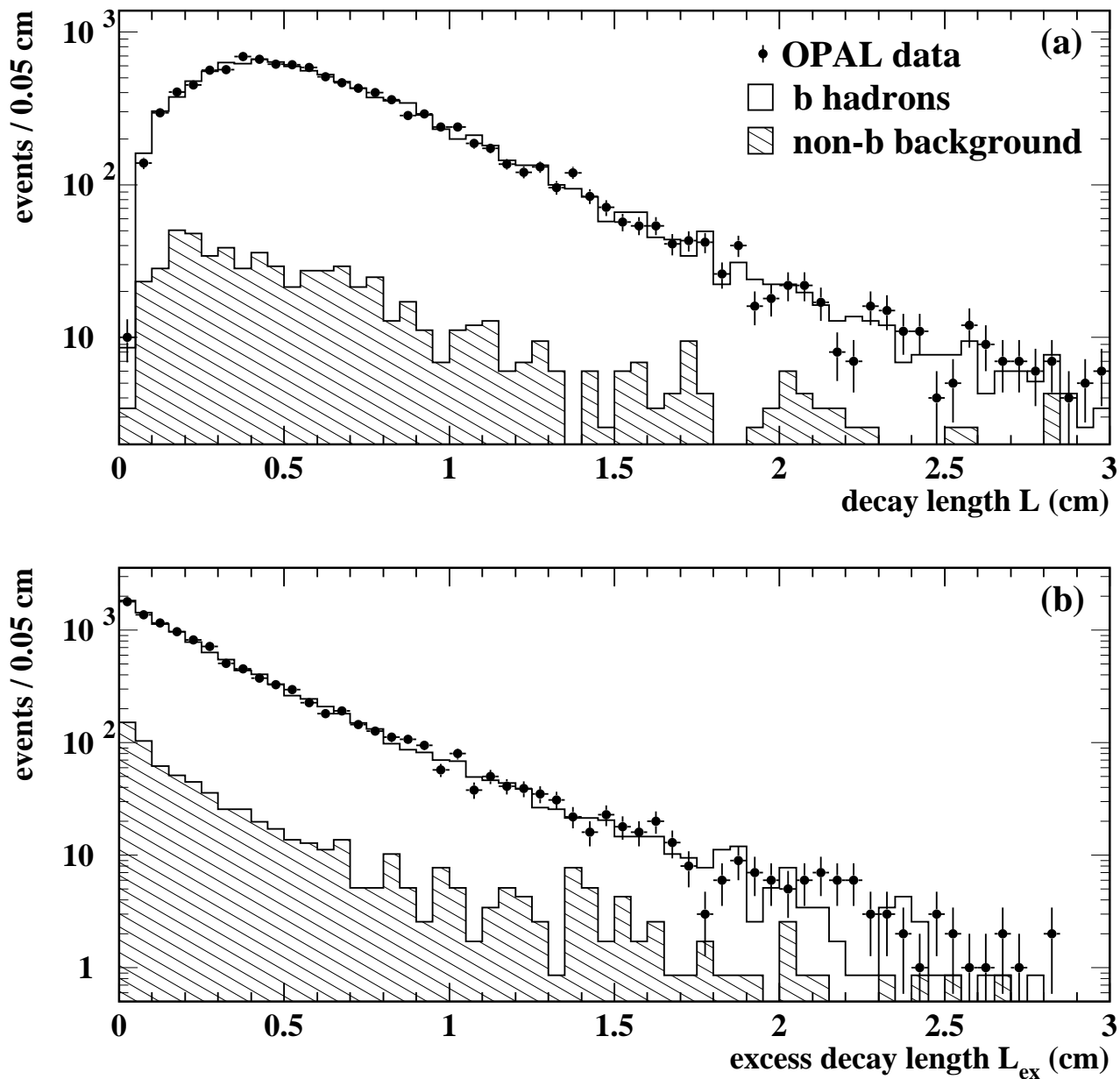
Figure 3: Distributions of (a) decay length L and (b) excess decay length L_{ex} in data (points with error bars) and Monte Carlo (histogram), for all selected secondary vertices. The expected contributions of b hadrons and non-b background are indicated.
