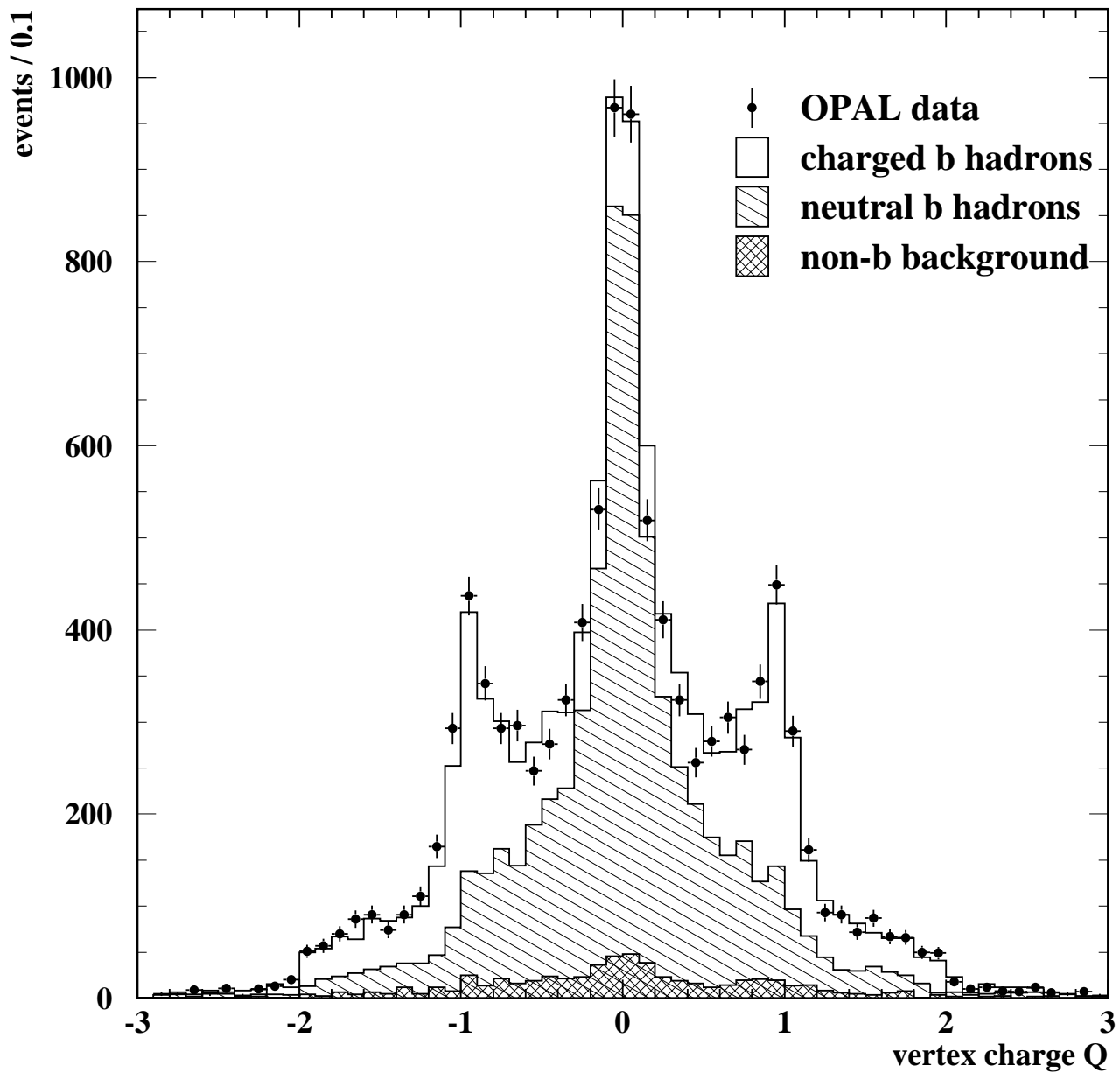
Figure 2: Distributions of the vertex charge Q in the data (points) and Monte Carlo (histogram), normalised to the same number of entries. The expected contributions from charged b hadrons, neutral b hadrons and non-b background are indicated.
