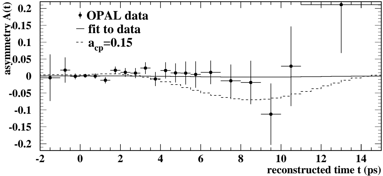
Figure 8: Asymmetry of tagged b and \bar{b} hadrons as a function of reconstructed time t in data (points), and fit (solid line). The expected asymmetry for a_{\text{cp}} = 0.15 is shown by the dotted line.
