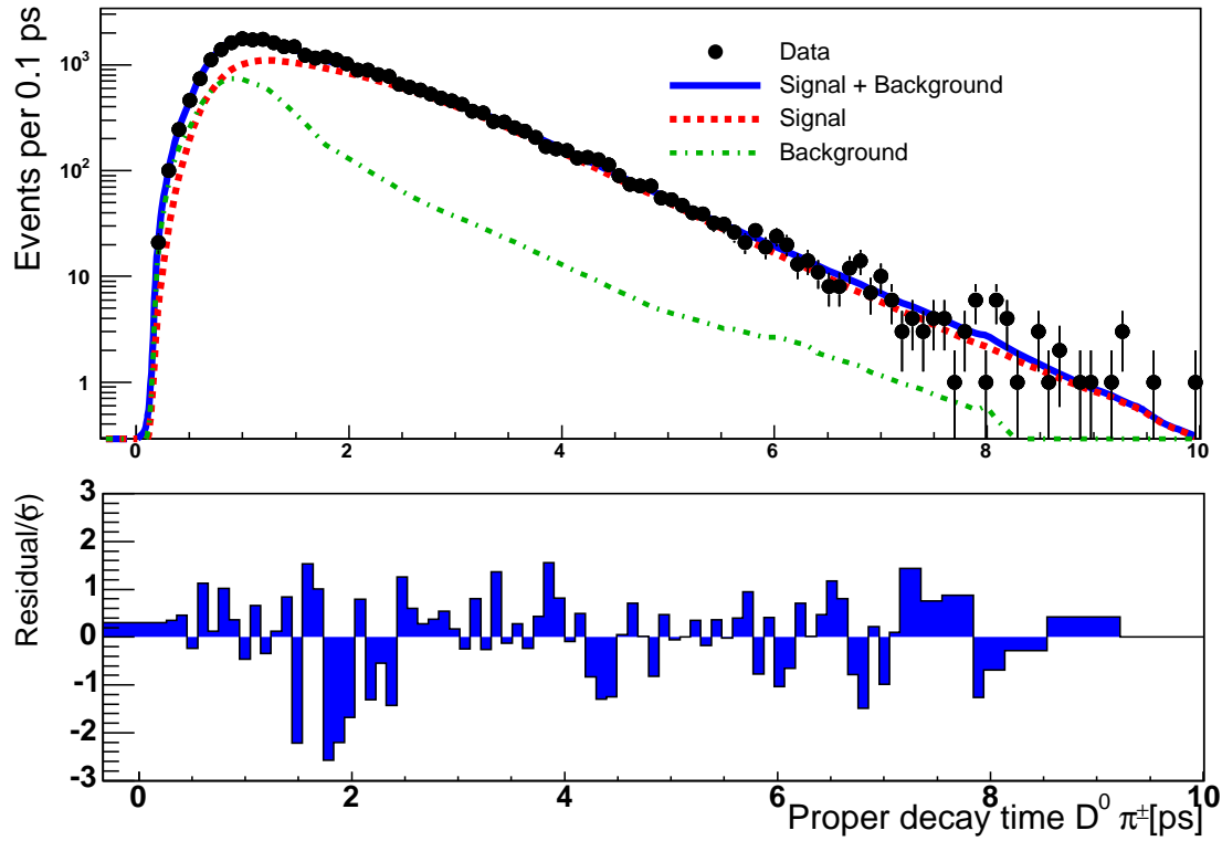
FIG. 8: This figure shows the projection of the lifetime fit onto the data. The signal and background components are shown separately (dotted lines) and in addition (solid line). The points are data. The lower plot shows the residual divided by the error for each bin.
