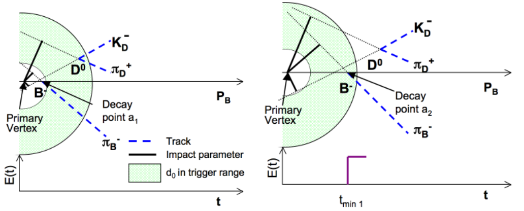
(a) If the decay occurs at point a_1 , only one track has an impact parameter within the trigger range (shaded region). E_i(t, \varepsilon_s) at the corresponding t is zero.
