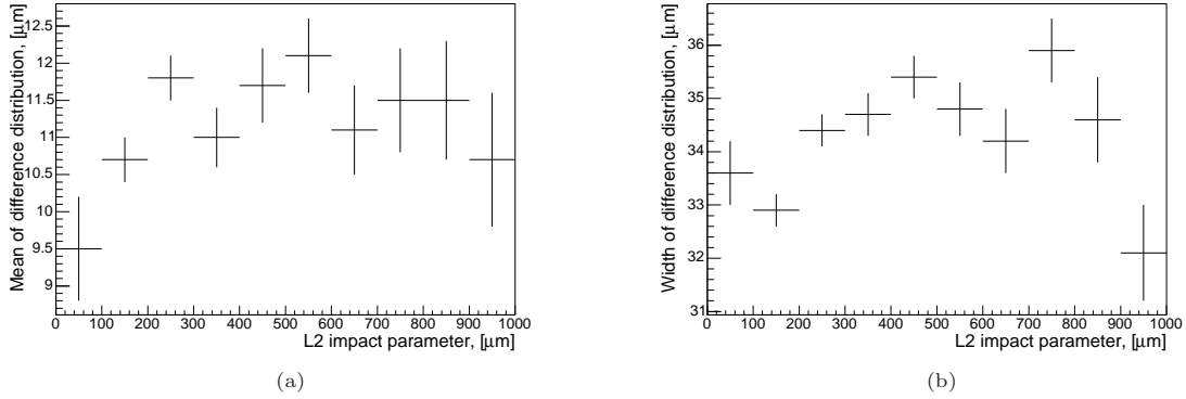
FIG. 3: The difference, (\Delta d_0)_{L2} is binned as a function of |d_0^{L2}| and fitted to a Gaussian. The mean of the fitted Gaussian is shown in (a) while the width is given in (b). The variation is of order a few microns.
