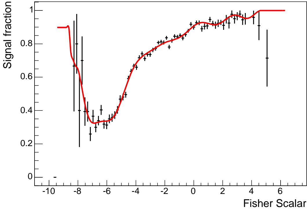
FIG. 7: The data points show the signal fraction as a function of Fisher scalar for a sample of simulated data. The line shows the projection of the Lagrange interpolating polynomial determined by the simultaneous fit to proper decay time, signal fraction and other parameters.
