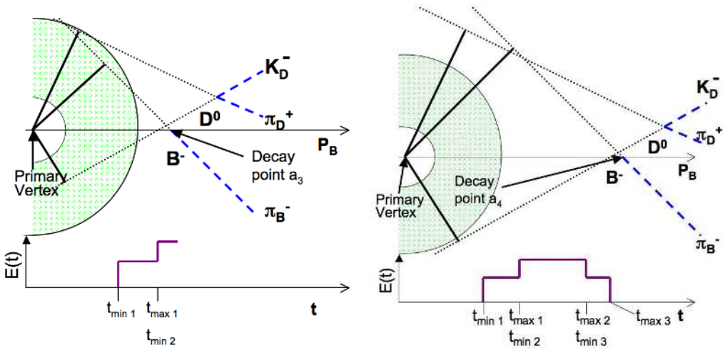
(c) If the decay occurs at a_3 there are two tracks pairs which would pass all trigger requirements. E_i(t, \varepsilon_s) rises at the point t_{min 2} as the probability to find at least one of the two available track pairs is greater than the probability to find a particular track pair.
