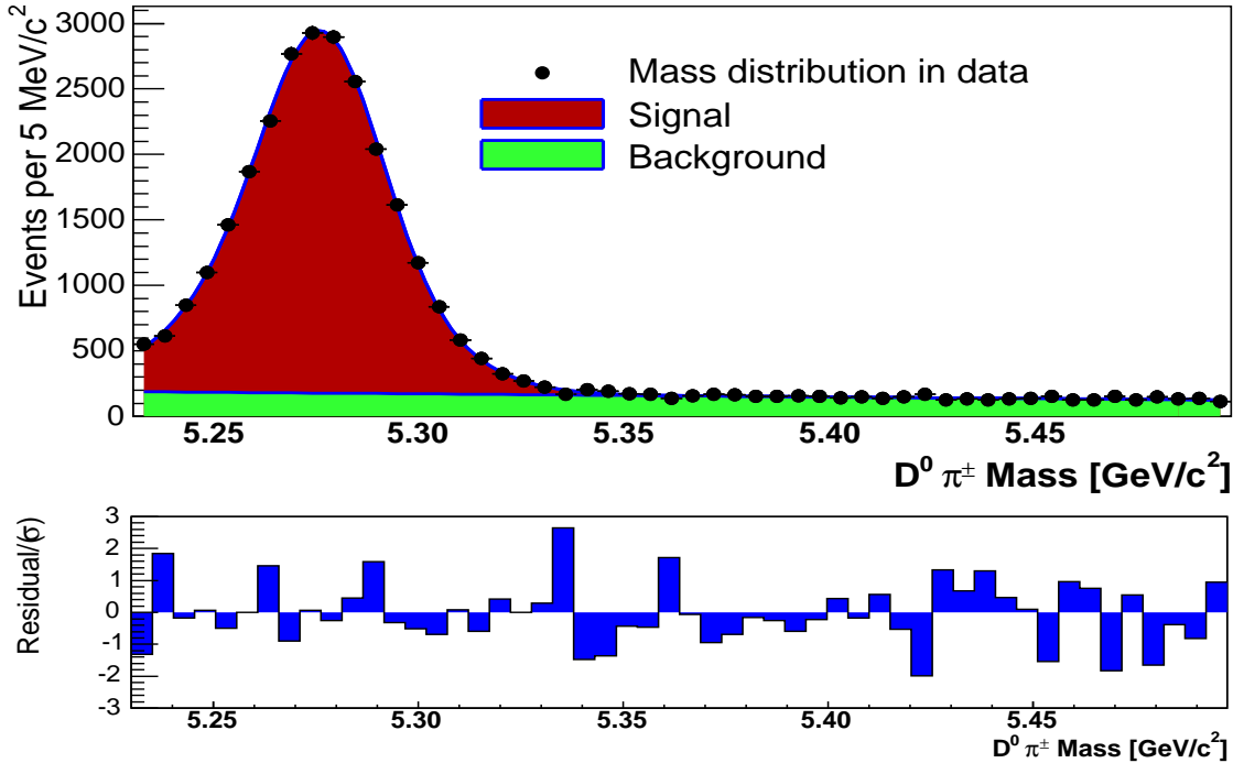
FIG. 1: The top plot shows the mass fit projection (line) on the data (points). The bottom plot shows the residual divided by the error for each bin: (N_{\text{fit}} - N_{\text{data}})/\sqrt{N_{\text{data}}} .
