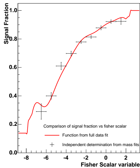
FIG. 9: Projection of the signal fraction, f(x) , as a function of the Fisher scalar, determined from the fit (line). The data points are the signal fraction determined from mass fits using events only lying in that particular bin of x .
