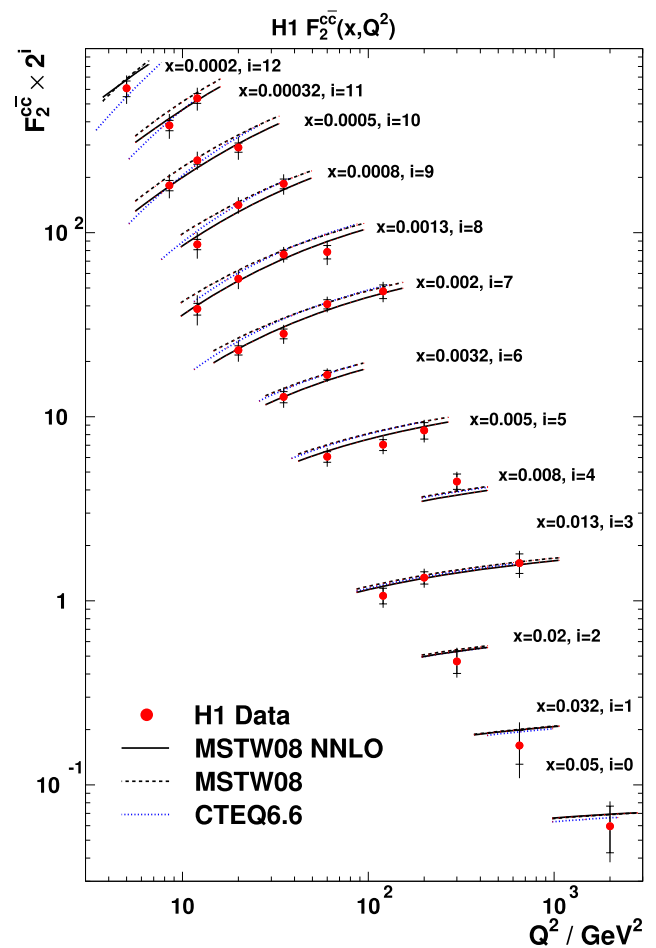
Fig. 17 The combined F_2^{c\bar{c}} shown as a function of Q^2 for various x values. The inner error bars show the statistical error, the outer error bars represent the statistical and systematic errors added in quadrature. The predictions of QCD calculations are also shown
