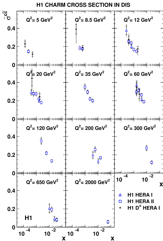
Fig. 11 The measured reduced cross section \tilde{\sigma}^{c\bar{c}} shown as a function of x for different Q^2 values. The inner error bars show the statistical error, the outer error bars represent the statistical and systematic errors added in quadrature. The HERA II measurements are compared with those from HERA I. The measurements obtained from D^* mesons by H1 [35] using HERA I data are also shown. The x values of the HERA I data are shifted for visual clarity
