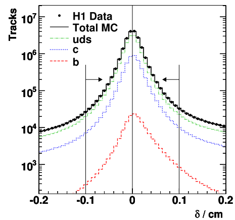
Fig. 2 The distribution of the signed impact parameter \delta of a track to the primary vertex in the X – Y plane. Included in the figure is the expectation from the Monte Carlo simulation for light, c and b quarks. The contributions from the various quark flavours in the Monte Carlo are shown after applying the scale factors \rho_l , \rho_c and \rho_b obtained from the fit to the complete data sample (see Sect. 4.4). The arrows indicate the range over which tracks are selected for analysis
