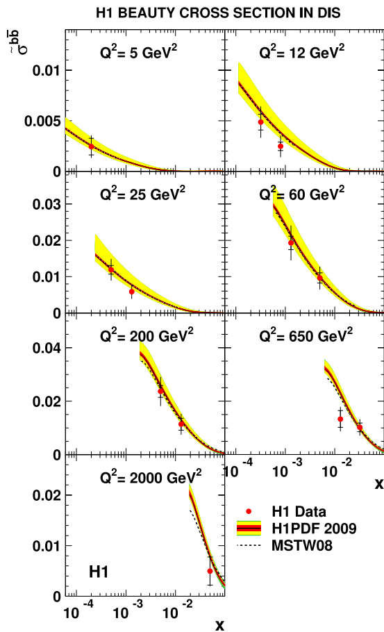
Fig. 16 The combined reduced cross section \bar{\sigma}^{b\bar{b}} (as in Fig. 15). The predictions of the H1PDF 2009 and MSTW08 NLO QCD fits are also shown. For the H1 QCD fit the inner error bands show the experimental uncertainty, the middle error bands include the theoretical model uncertainties of the fit assumptions, and the outer error band represents the total uncertainty including the parameterisation uncertainty
