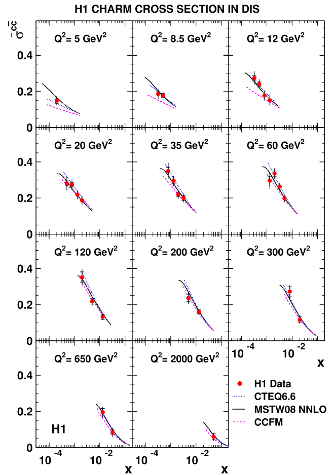
Fig. 13 The combined reduced cross section \tilde{\sigma}^{c\bar{c}} shown as a function of x for different Q^2 values. The inner error bars show the statistical error, the outer error bars represent the statistical and systematic errors added in quadrature. The predictions of QCD calculations are also shown
