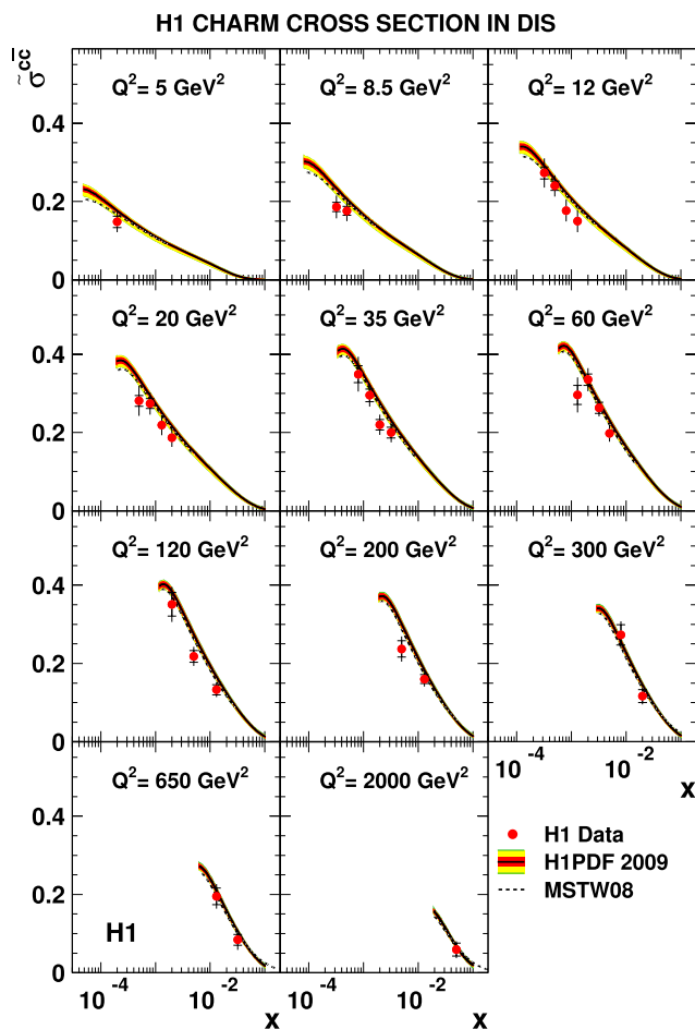
Fig. 14 The combined reduced cross section \tilde{\sigma}^{c\bar{c}} (as in Fig. 13). The predictions of the H1PDF 2009 and MSTW08 NLO QCD fits are also shown. For the H1 QCD fit the inner error bands show the experimental uncertainty, the middle error bands include the theoretical model uncertainties of the fit assumptions, and the outer error band represents the total uncertainty including the parameterisation uncertainty
