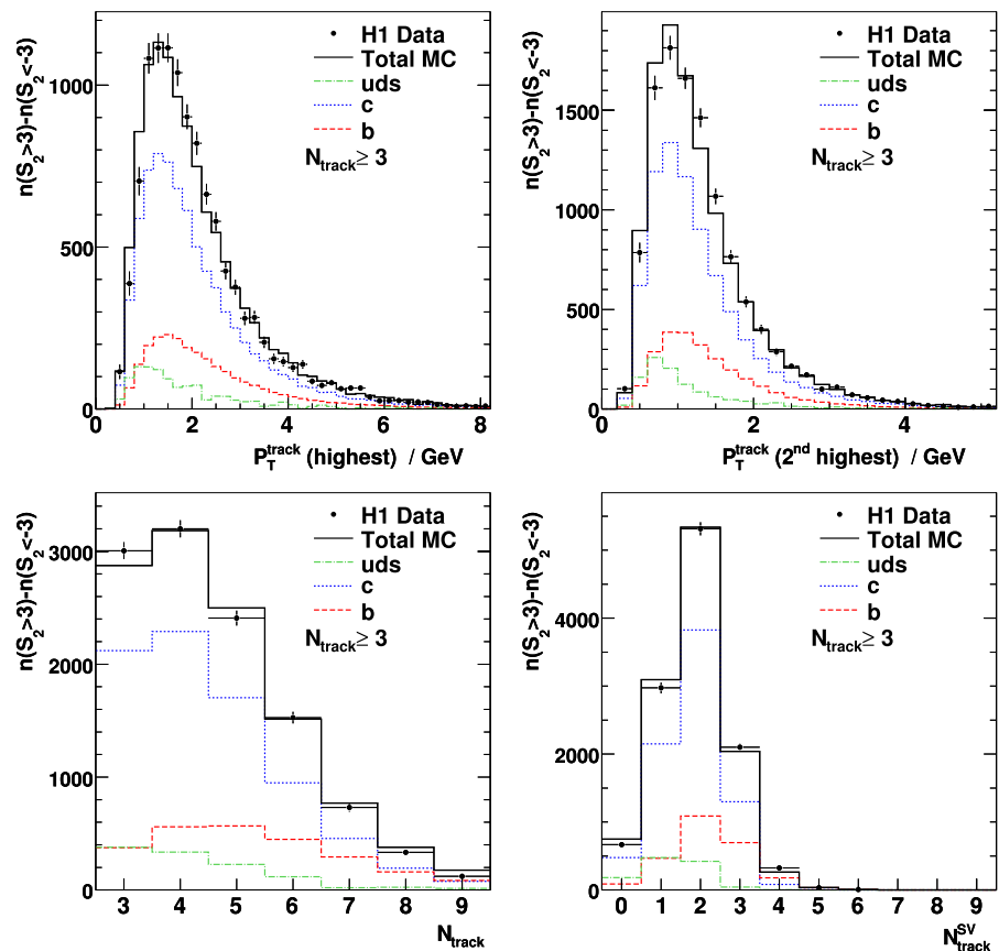
Fig. 7 The subtracted distributions for P_T^{\text{track}} of the highest and second highest transverse momentum track, N_{\text{track}} and N_{\text{track}}^{\text{SV}} . Each plot shows the difference between the distributions for those events with S_2 > 3 and the corresponding distribution with S_2 < -3 . Included in the figure is the expectation from the Monte Carlo simulation for light, c and b quarks. The contributions from the various quark flavours in the Monte Carlo are shown after applying the scale factors \rho_l , \rho_c and \rho_b obtained from the fit to the complete data sample
