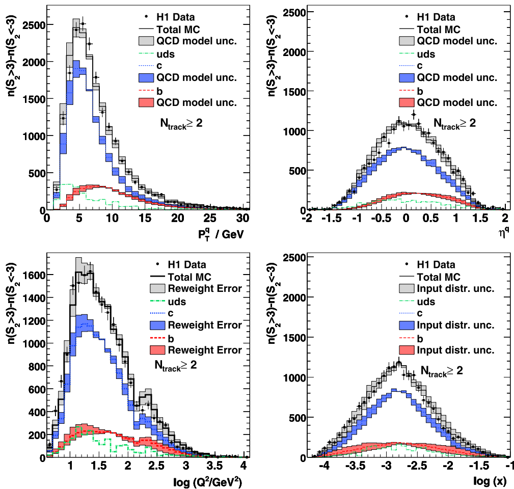
Fig. 8 The subtracted distributions for P_T^q , \eta^q , \log Q^2 , \log x . Each plot shows the difference between the distributions for those events with S_2 > 3 and the corresponding distribution with S_2 < -3 . Included in the figure is the expectation from the Monte Carlo simulation for light, c and b quarks. The contributions from the various quark flavours in the Monte Carlo are shown after applying the scale factors \rho_l , \rho_c and
