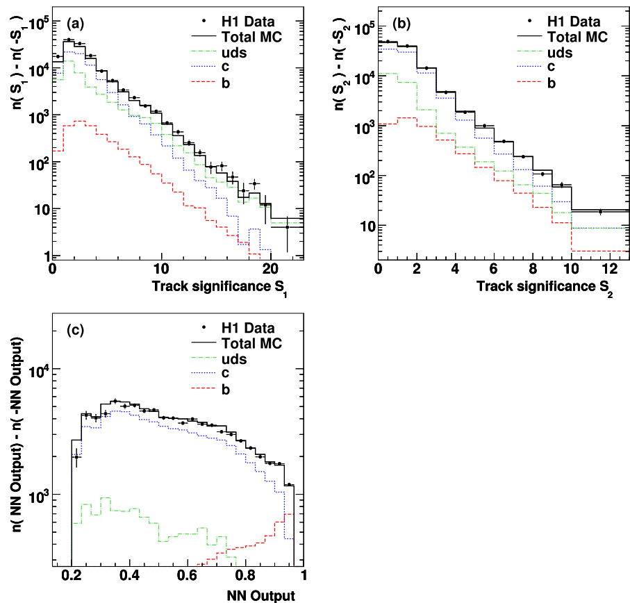
Fig. 9 The output of the NN. Included in the figure is the expectation from the Monte Carlo simulation for light, c and b quarks. The contributions from the various quark flavours in the Monte Carlo are shown after applying the scale factors \rho_l , \rho_c and \rho_b obtained from the fit to the complete data sample
