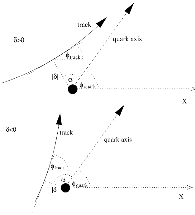
Fig. 1 Diagrams of a track in the X – Y plane. If the angle \alpha is less than 90^\circ , \delta is defined as positive otherwise \delta is defined as negative
