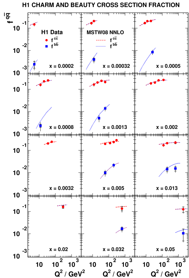
Fig. 19 The charm and beauty contributions to the total cross section, f^{c\bar{c}} and f^{b\bar{b}} , shown as a function of Q^2 for different x values. The inner error bars show the statistical error, the outer error bars represent the statistical and systematic errors added in quadrature. A prediction of NNLO QCD is also shown. The charm data point at x = 0.005 and Q^2 = 300 \text{ GeV}^2 has been interpolated from x = 0.008
