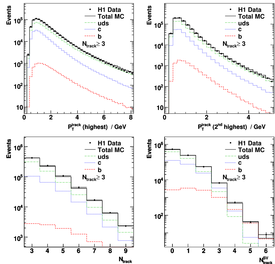
Fig. 5 Inputs to the NN for events with at least 3 CST tracks: p_T^{\text{track}} of the highest and second highest transverse momentum track, N_{\text{track}} and N_{\text{track}}^{\text{SV}} . Included in the figure is the expectation from the Monte Carlo simulation for light, c and b quarks. The contributions from the various quark flavours in the Monte Carlo are shown after applying the scale factors \rho_l , \rho_c and \rho_b obtained from the fit to the complete data sample
