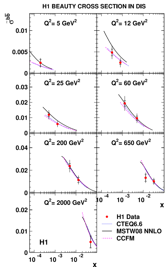
Fig. 15 The combined reduced cross section \tilde{\sigma}^{b\bar{b}} shown as a function of x for different Q^2 values. The inner error bars show the statistical error, the outer error bars represent the statistical and systematic errors added in quadrature. The predictions of QCD calculations are also shown
