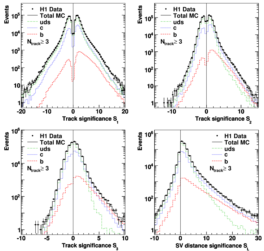
Fig. 4 Inputs to the NN for events with at least 3 CST tracks: |S_1| , |S_2| , |S_3| and S_L . Included in the figure is the expectation from the Monte Carlo simulation for light, c and b quarks. The contributions from the various quark flavours in the Monte Carlo are shown after applying the scale factors \rho_l , \rho_c and \rho_b obtained from the fit to the complete data sample
