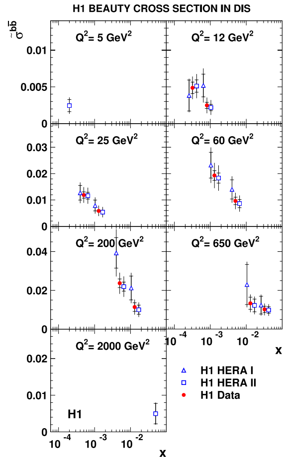
Fig. 12 The measured reduced cross section \tilde{\sigma}^{b\bar{b}} shown as a function of x for different Q^2 values. The inner error bars show the statistical error, the outer error bars represent the statistical and systematic errors added in quadrature. The HERA II measurements are compared with those from HERA I. The combined H1 data are also shown. The x values of the HERA I and HERA II data are shifted for visual clarity
