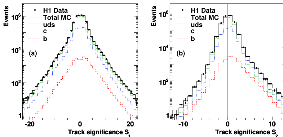
Fig. 3 The significance \delta/\sigma(\delta) distribution (a) of the highest absolute significance track ( S_1 ) and (b) of the track with the second highest absolute significance ( S_2 ). Included in the figure is the expectation from the Monte Carlo simulation for light, c and b quarks. The contributions from the various quark flavours in the Monte Carlo are shown after applying the scale factors \rho_l , \rho_c and \rho_b obtained from the fit to the complete data sample
