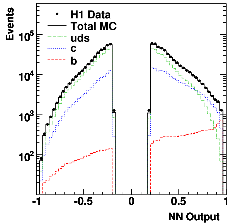
Fig. 9 The output of the NN. Included in the figure is the expectation from the Monte Carlo simulation for light, c and b quarks. The contributions from the various quark flavours in the Monte Carlo are shown after applying the scale factors \rho_l , \rho_c and \rho_b obtained from the fit to the complete data sample
