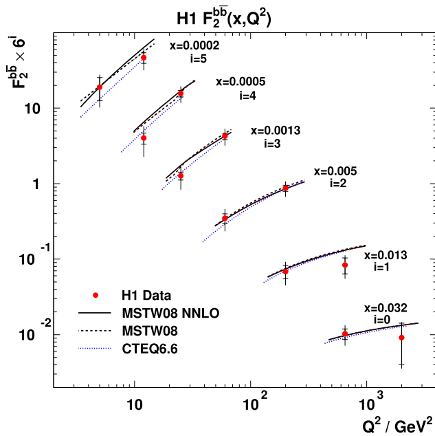
Fig. 18 The combined F_2^{b\bar{b}} shown as a function of Q^2 for various x values. The inner error bars show the statistical error, the outer error bars represent the statistical and systematic errors added in quadrature. The predictions of QCD calculations are also shown. Note that some points have been interpolated in x for visual clarity
