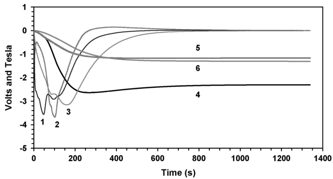
Fig. 5. Voltages (curves 1, 2, and 3) induced in steel blocks of the barrel next to central wheel in the inner (1), middle (2), and outer (3) layers during the coil "fast" discharge from full current of 19140 A to zero and integrated magnetic flux densities (curves 4, 5, and 6) in the inner (4), middle (5), and outer (6) layers.
