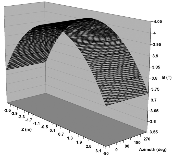
Fig. 2. Magnetic flux density measured at radius 92 mm along the coil axis in the range of \pm 3.5 m with respect to the coil middle plane for full azimuth coverage.
