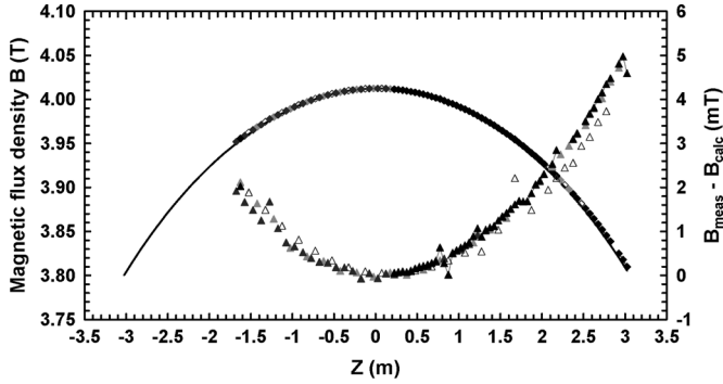
Fig. 3. Magnetic flux density (left scale) measured at the coil axis with NMR probe (rhombuses) in the range from -1.675 to 3.025 m with respect to the coil middle plane. Smooth curve represents the calculations done with the CMS TOSCA model. The triangles show the difference between the measured and calculated B values (right scale). The model is normalized to get the measured B_0 value 4.0124 T. Different colors mark four different sets of the measurements when the fieldmapper traveled in both axial directions.
