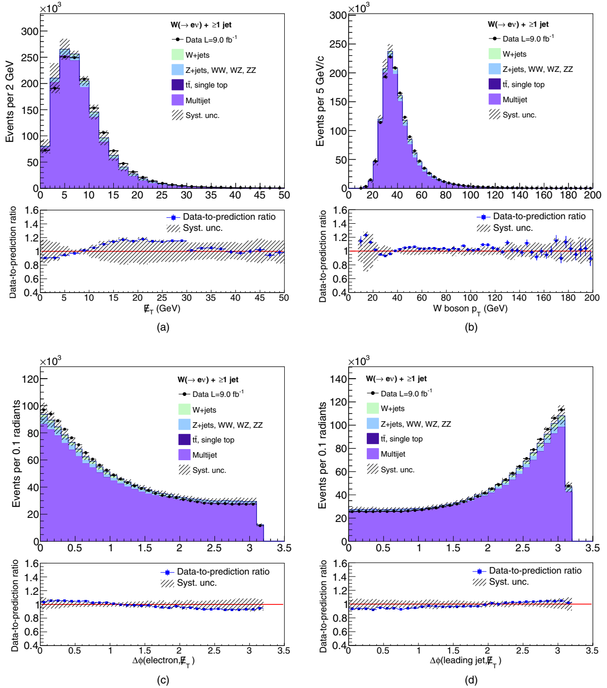
FIG. 10. Validation plots of the background model in the electron channel: comparison between the data and the prediction for the distributions of (a) missing transverse energy \cancel{E}_T , (b) W -boson p_T , (c) azimuthal distance between the electron and the \cancel{E}_T [ \Delta\phi(e, \cancel{E}_T) ], and (d) azimuthal distance between the leading jet and the \cancel{E}_T [ \Delta\phi(\text{leading jet}, \cancel{E}_T) ] in the control region. The data are represented by the black points while the signal and the background predictions are represented by stacked histograms. Systematic uncertainties on the predictions are indicated by the shaded areas (see Sec. IV for discussion on systematic uncertainty). The lower plots show the ratios between the data and the corresponding predictions.
