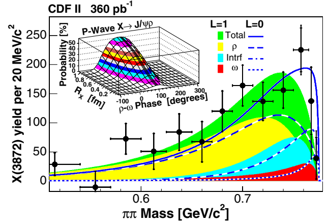
FIG. 4 (color online). A blowup of the X(3872) spectrum with J/\psi\rho fits which include \rho - \omega interference ( 95^\circ phase) with relative amplitudes set by \mathcal{R}_{3/2} = 1.0 . Fits for both L = 0 (lines) and 1 (shaded regions) are shown, along with their decomposition into \rho , \omega , and interference terms. The inset shows L = 1 fit probabilities as a function of \phi and R_X in 5% contours.
