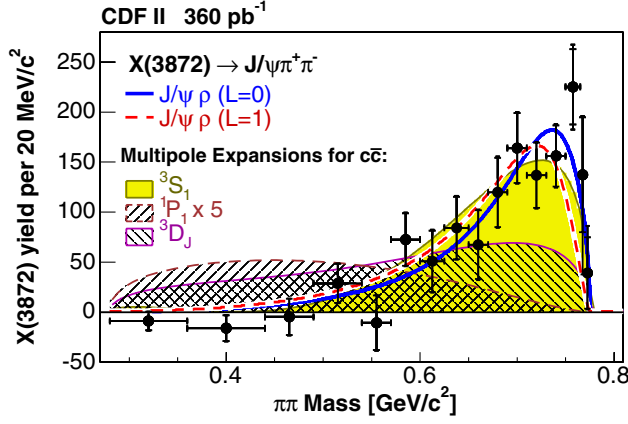
FIG. 3 (color online). The dipion mass spectrum for the X(3872) \rightarrow J/\psi\pi^+\pi^- and fits to various hypotheses (see text). The fitted curve for the {}^1P_1 model is scaled up by a factor of 5 for better visibility.
