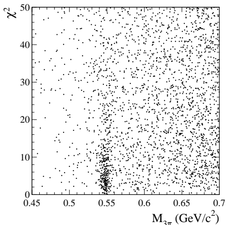
FIG. 7: Scatter plot of \chi^2_{3\pi\gamma\gamma} versus M_{3\pi} for the selected data events containing an additional photon.
