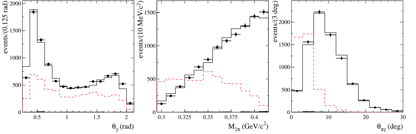
FIG. 11: Distributions of the photon polar angle (left), the invariant mass of the two charged pions (middle), and the minimum angle between a charged pion and a photon from the \pi^0 decay (right) for data (points with error bars) and simulated (solid lines) e^+e^- \rightarrow \gamma_{ISR}\omega events. The simulated background is shown as the (very small) shaded histograms, and the dashed lines show the distributions for simulated e^+e^- \rightarrow \eta\gamma events.
