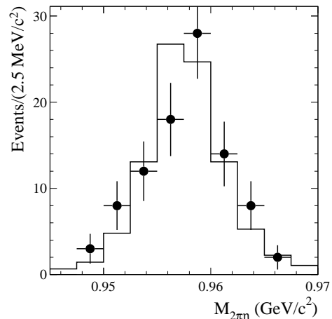
FIG. 9: Distributions of the \pi^+\pi^-\eta invariant mass for selected e^+e^-\rightarrow\gamma_{ISR}J/\psi\rightarrow\gamma_{ISR}\eta'\gamma events in the data (points with error bars) and simulation (histogram).
