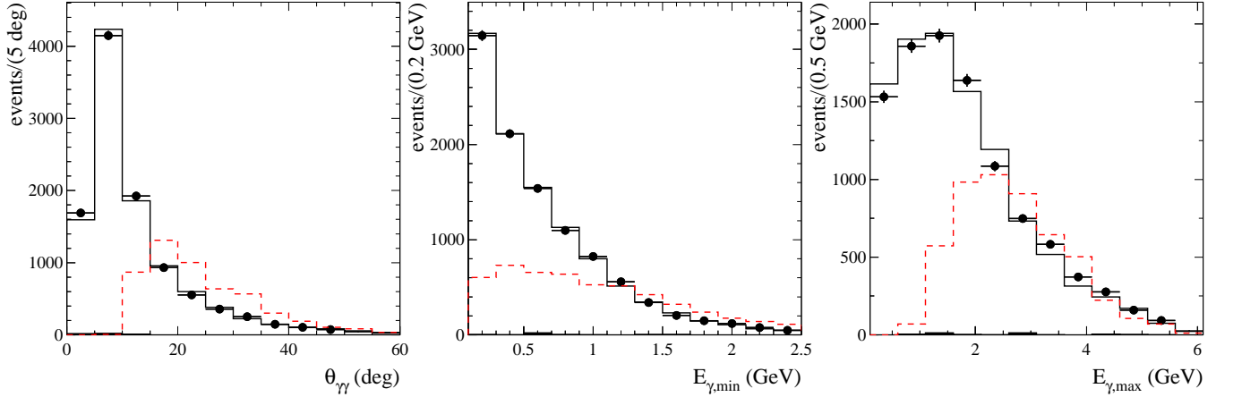
FIG. 12: Distributions of the angle between the two photons from the \pi^0 \rightarrow \gamma\gamma or \eta \rightarrow \gamma\gamma decay (left), and the minimum (middle) and maximum (right) energy of the decay photons, for data (points with error bars) and simulated (solid lines) e^+e^- \rightarrow \gamma_{ISR}\omega events, simulated background events (small shaded histograms), and simulated e^+e^- \rightarrow \eta'\gamma \rightarrow \pi^+\pi^-\eta events (dashed lines).
