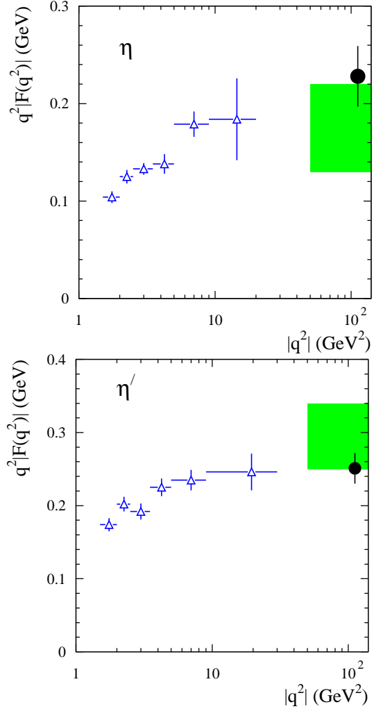
FIG. 13: The magnitudes of the \eta\gamma (top) and \eta'\gamma (bottom) transition form factors measured in this work (filled circle) and by CLEO [13] (triangles). The shaded boxes indicate the ranges of form-factor values calculated according to Eq.(2) with the decay constants from Refs. [3–8].
