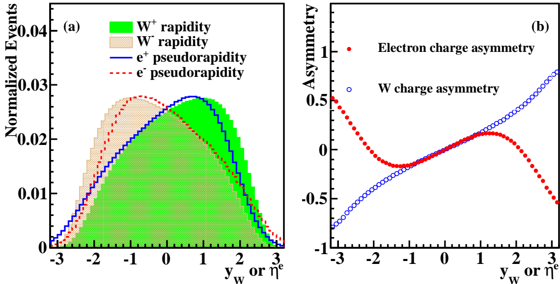
FIG. 1: (color online). (a) The W boson rapidity ( y_W ) and electron pseudorapidity ( \eta^e ) distributions in p\bar{p} collisions. (b) The charge asymmetry for the W boson and the decay electron. The electron asymmetry has a “turn-over” due to the convolution of the W boson asymmetry and the V - A structure of the W boson decay. These predictions were obtained using the MC event generator RESBOS [5] with the CTEQ6.6 [6] central PDF set, using the kinematic cuts p_T^e > 25 GeV and p_T^W > 25 GeV.
