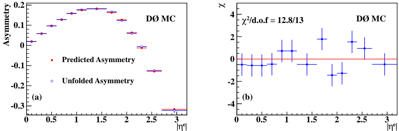
FIG. 10: (color online). (a) Closure test I of the unfolding method for the kinematic bin E_T^e > 25 GeV, E_T^{\text{miss}} > 25 GeV, using half of the MC sample as input for the unfolding procedure and the other half as pseudo data. The solid red points are the PYTHIA generator-level electron asymmetries and the open blue points are the unfolded asymmetries. The asymmetries are shown after CP-folding. (b) \chi distribution between predicted asymmetry and unfolded asymmetry, where \chi_i = \Delta A_i / \sigma_i , \Delta A_i is the difference between the generator-level asymmetry and the unfolded asymmetry, and \sigma_i is the statistical uncertainty in bin i .
