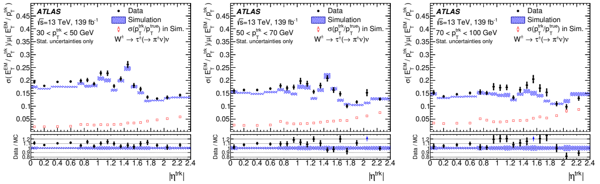
Figure 9: The fitted width divided by the mean of the E_T^{EM}/p_T^{\text{trk}} distribution as a function of the track |\eta| in three p_T^{\text{trk}} ranges: 30 < p_T^{\text{trk}} < 50 GeV, 50 < p_T^{\text{trk}} < 70 GeV and 70 < p_T^{\text{trk}} < 100 GeV. Also shown is the fitted width of the track p_T divided by the generator-level p_T for true \tau \rightarrow \pi^\pm \nu events in simulation to give an illustration of the contribution to the total width from the resolution of reconstructed tracks. The uncertainties shown are only those from the limited number of events in the dataset and simulated samples.
