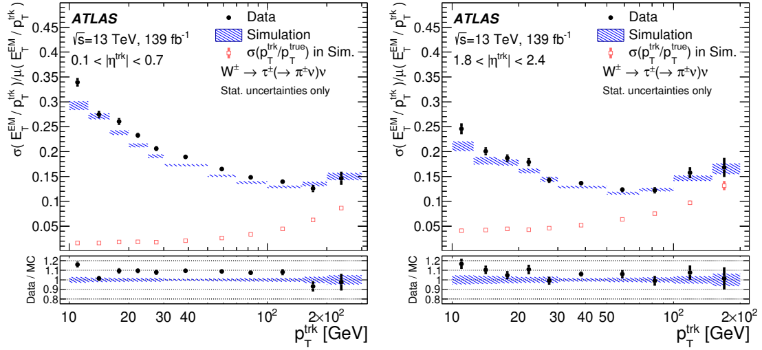
Figure 8: The fitted width divided by the mean of the E_T^{EM}/p_T^{\text{trk}} distribution as a function of the track p_T in the central region (left) and endcap region (right). Also shown is the fitted width of the track p_T divided by the generator-level p_T for true \tau \rightarrow \pi^\pm \nu events in simulation to give an illustration of the contribution to the total width from the resolution of reconstructed tracks. The uncertainties shown are only those from the limited number of events in the dataset and simulated samples.
