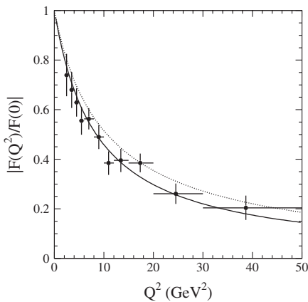
FIG. 26. The \gamma\gamma^* \rightarrow \eta_c transition form factor normalized to F(0) (points with error bars). The solid curve shows the fit to Eq. (22). The dotted curve shows the leading order pQCD prediction from Ref. [3].
