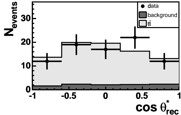
FIG. 1: Measured \cos \theta_{\text{rec}}^* distribution shown together with the estimated signal and background. The t\bar{t} signal events are modeled by the standard model Monte Carlo generator PYTHIA with m_t = 178 \text{ GeV}/c^2 .
