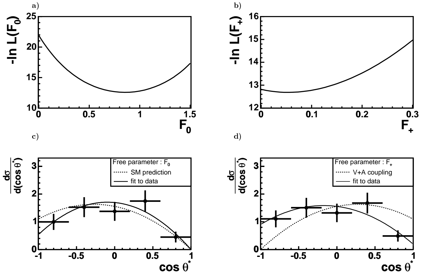
FIG. 2: Extraction of the longitudinal ( F_0 ) and right-handed ( F_+ ) fraction. For both fits F_0 and F_+ are used as single free parameter. In each case the other parameter is set to its expected standard model value. a,b) Negative log likelihood as a function of F_0 or F_+ . c,d) Binned \cos \theta^* distribution for data, corrected for acceptance and reconstruction effects. The distributions corresponding to the fit results F_0 = 0.85 and F_+ = 0.05 are shown as a continuous functions. The dashed curve shows the theoretical prediction for F_0 = 0.7 or for F_+ = 0.3 .
