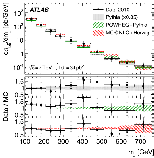
Fig. 6 The b\bar{b} -dijet cross-section as a function of dijet invariant mass for b -jets with p_T > 40 GeV and |y| < 2.1 . The data are compared to the MC predictions of Pythia, POWHEG and MC@NLO. The leading-order Pythia prediction is scaled to the measured integrated cross-section. The shaded regions around the MC predictions reflect the statistical uncertainty only
