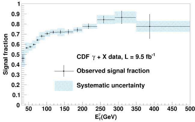
FIG. 2. Signal fraction as a function of leading-photon E_T . The points are plotted at the average E_T^\gamma of the data within each bin. The error bars represent the statistical uncertainty, while bands represent the total systematic uncertainty.
