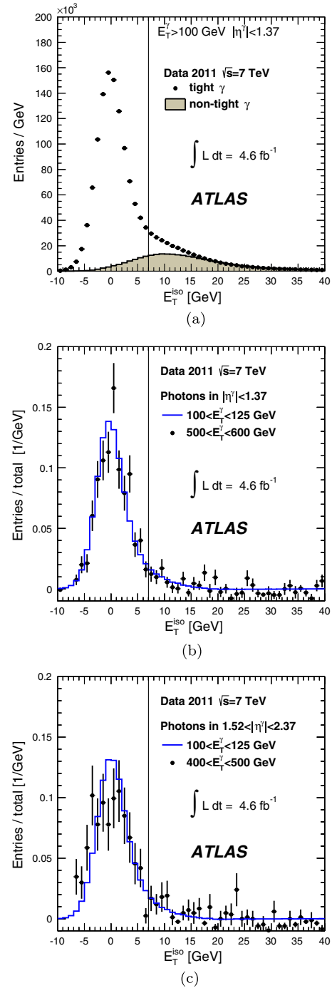
FIG. 1 (color online). (a) Distributions of tight photon transverse energy E_T^{\text{iso}} (dots) and nontight (shaded gray region) photon candidates in data, for photon transverse energy E_T^{\text{iso}} > 100 GeV in the central \eta' region. The latter is normalized to the former for E_T^{\text{iso}} > 15 GeV. Distributions of tight E_T^{\text{iso}} photons in the barrel (b) and end-cap (c) regions after subtracting the normalized nontight distribution. For both (b) and (c) a comparison of two representative E_T^{\text{iso}} regions with different \eta' is shown. The vertical lines show the requirement of E_T^{\text{iso}} \leq 7 GeV used to define the final cross sections. These distributions are normalized to one.
