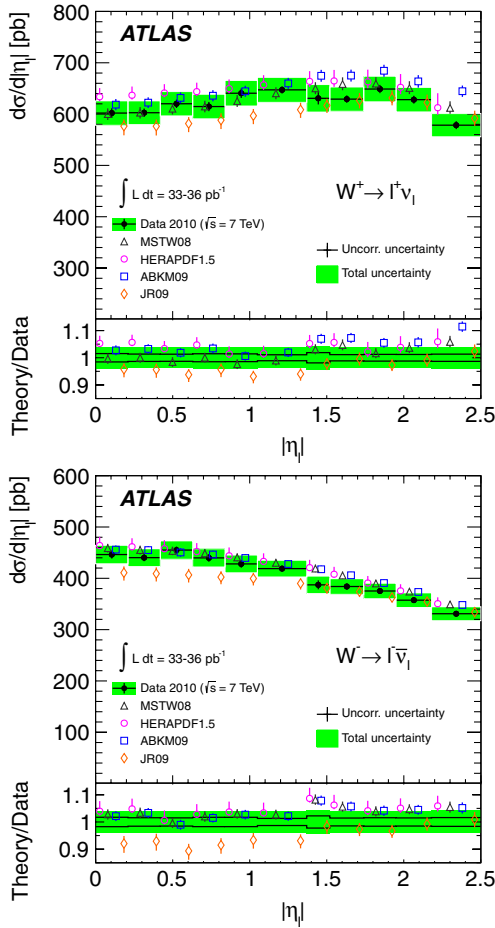
FIG. 13 (color online). Differential d\sigma/d|\eta_{\ell^\pm}| (top panel) and d\sigma/d|\eta_{\ell^\mp}| (bottom panel) cross section measurements for W \rightarrow \ell\nu compared to the NNLO theory predictions using various PDF sets. The kinematic requirements are p_{T,\ell} > 20 GeV, p_{T,\nu} > 25 GeV, and m_T > 40 GeV. The ratio of theoretical predictions to data is also shown. Theoretical points are displaced for clarity within each bin.
