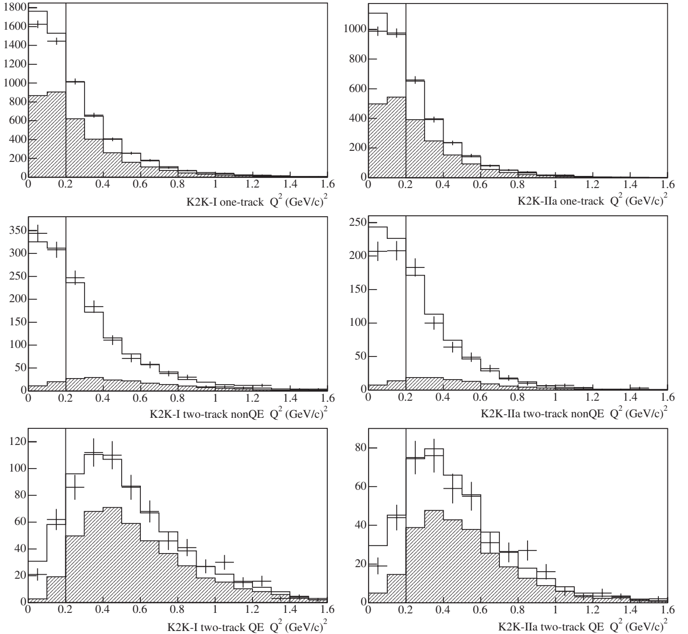
FIG. 7. The data and the best fit Q^2_{\text{rec}} distributions for K2K-I data (left) and K2K-IIa data (right) for the one-track, two-track QE enhanced, and two-track non-QE enhanced samples. The shaded region shows the QE fraction of each sample, estimated from the MC. The contribution from each energy region is summed for each plot. The lowest two data points in each plot are not included in the fit, due to the large uncertainty in the effects of the nucleus.
