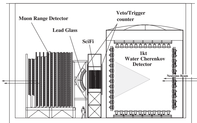
FIG. 1. The arrangement of the near neutrino detectors at KEK. The beam comes in from the right and continues to Super-Kamiokande, 250 km away to the left. The SciFi detector is on a stand in the middle.
