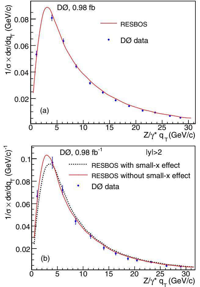
FIG. 1 (color online). The normalized differential cross section as a function of q_T for (a) the inclusive sample and (b) the sample with Z boson |y| > 2 with q_T < 30 \text{ GeV}/c . The points are the data, the solid curve is the RESBOS prediction, and the dashed line in (b) is the prediction from the form factor modified after studies of small- x DIS data.
