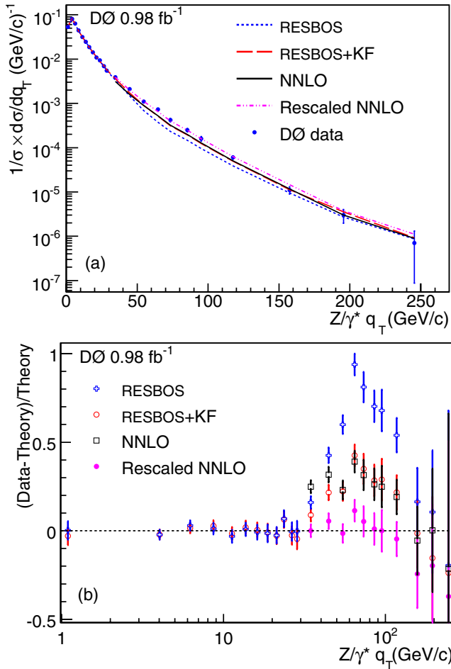
FIG. 2 (color online). The normalized differential cross section as a function of q_T compared to four theoretical calculations for (a) the entire range measured and (b) the fractional differences between data and the theoretical predictions. The four theoretical calculations are RESBOS with its default parameters, RESBOS with a NLO to NNLO K factor by Arnold and Reno, the NNLO calculation by Melnikov and Petriello, and the NNLO calculation but rescaled to data at q_T = 30 GeV/ c .
