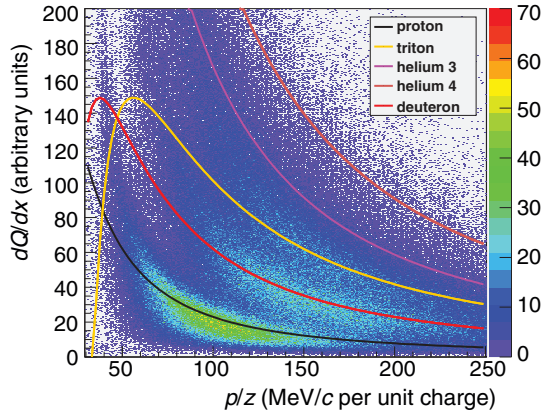
FIG. 7. (Color online) The ionization density distribution of particles registered by the RTPC after the RTPC gain calibration. The solid curves are calculated based on the Bethe-Bloch formula for dE/dx for various particles, in order from bottom to top: proton, deuteron, triton, helion ( {}^3\text{He} ), \alpha ( {}^4\text{He} ). The target was filled with {}^4\text{He} gas and the electron energy was 2 GeV for this measurement.
