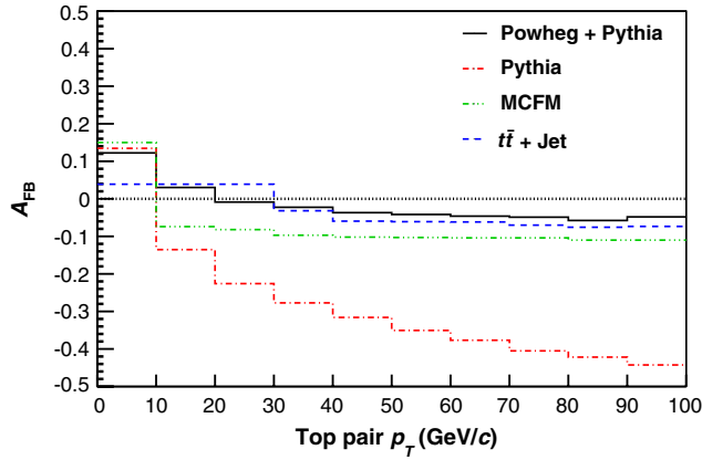
FIG. 22 (color online). Expected A_{\text{FB}} as a function of the p_T^{t\bar{t}} of the t\bar{t} system at the parton level from MCFM, POWHEG, and PYTHIA, as well as a NLO prediction for events where the top-quark pair is produced in association with an extra energetic jet.
