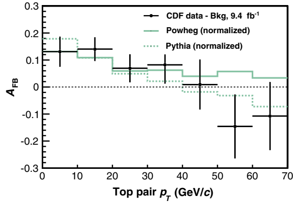
FIG. 25 (color online). The background-subtracted forward-backward asymmetry in the data as a function of the transverse momentum of the t\bar{t} system, compared to both POWHEG and PYTHIA. The model predictions have been normalized by the addition of \Delta A_{\text{NLO}} to POWHEG and \Delta A_{\text{LO}} to PYTHIA as described in the text. Error bars include both statistical and background-related systematic uncertainties. The last bin contains overflow events.
