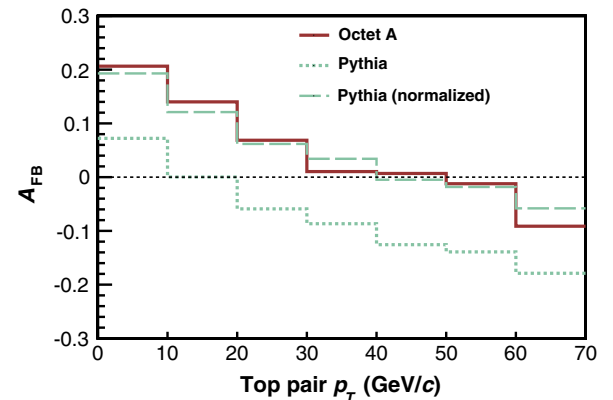
FIG. 24 (color online). The forward-backward asymmetry as a function of the transverse momentum of the t\bar{t} system for three models at the background-subtracted level: Octet A, SM PYTHIA, and SM PYTHIA normalized by the addition of \Delta A_{\text{Oct}} . The last bin contains overflow events.
