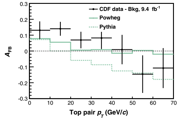
FIG. 23 (color online). The background-subtracted forward-backward asymmetry in the data as a function of the transverse momentum of the t\bar{t} system, compared to both POWHEG and PYTHIA. Error bars include both statistical and background-related systematic uncertainties. The last bin contains overflow events.
