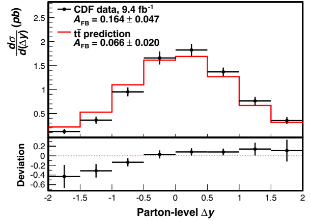
FIG. 13 (color online). (top) The differential cross section d\sigma/d(\Delta y) as measured in the data after correction to the parton level compared to the SM prediction. Uncertainties include both statistical and systematic contributions and are correlated between bins. (bottom) The difference between the data and prediction divided by the prediction.
