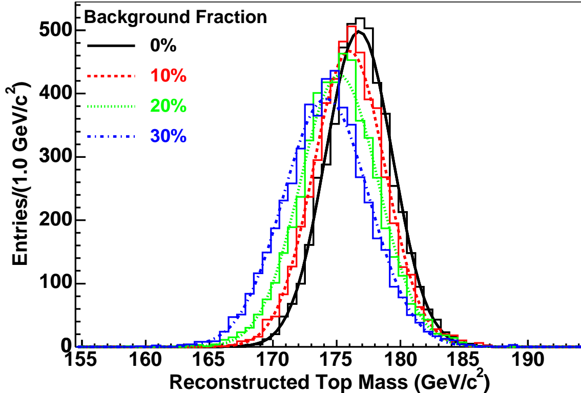
FIG. 11: An example of mass shift due to background events. The plot shows the reconstructed mass (input M_{top} = 178 \text{ GeV}/c^2 ), varying the background fraction from 0% to 30% (expected fraction is 14.5%). For each distribution, 5000 sets of pseudo-experiments that contain 63 events each are performed. Each distribution is fitted with a Gaussian function.
