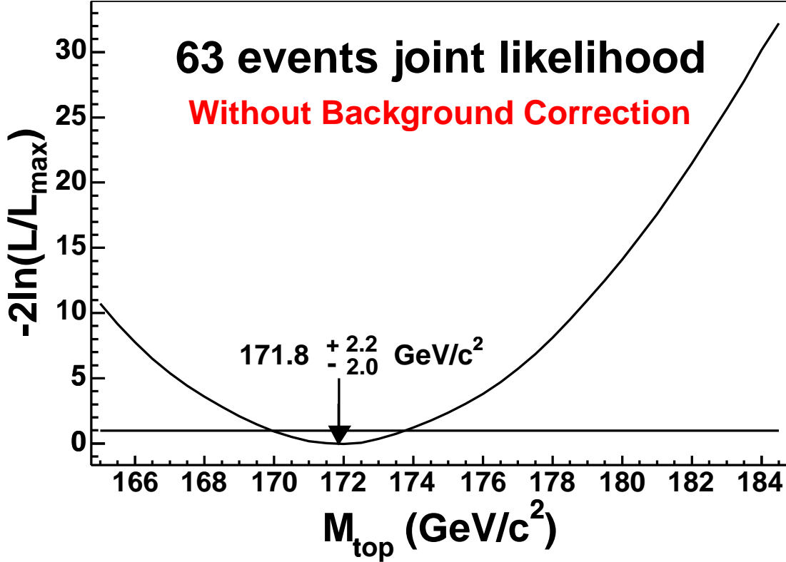
FIG. 16: The joint negative log likelihood distribution of the 63 events observed in the data. The fit gives M_{\text{top}} = 171.8 \begin{smallmatrix} +2.2 \\ -2.0 \end{smallmatrix} \text{ GeV}/c^2 , before any corrections.
