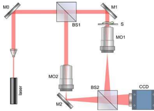
Fig. 1. DHM setup. M's: mirrors; BS's: beam splitters; MO's: microscope objectives; S: sample object
