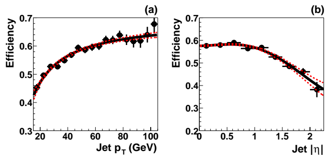
FIG. 7: Semileptonic b tagging efficiency vs. (a) jet p_T and (b) jet |\eta| measured in a b\bar{b} MC sample. The resulting fit is shown as a solid line, and the \pm 1\sigma statistical uncertainty is shown as dotted lines.
