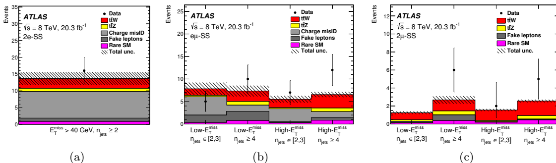
Figure 5. Event yields in the same-sign dilepton signal regions according to the binning used in the final likelihood fit in the (a) 2e -SS (b) e\mu -SS and (c) 2\mu -SS regions. The distributions are shown before the fit. The bins labelled “Low- E_T^{\text{miss}} ” correspond to E_T^{\text{miss}} \in (40, 80) GeV, and those labelled “High- E_T^{\text{miss}} ” correspond to E_T^{\text{miss}} \geq 80 GeV. “Rare SM” contains small background contributions mainly consisting of the t\bar{t}H and WZ processes. Instrumental backgrounds, including fake leptons and leptons with misidentified charge are predicted using data-driven methods. The hatched area corresponds to the total uncertainty on the predicted yields.
