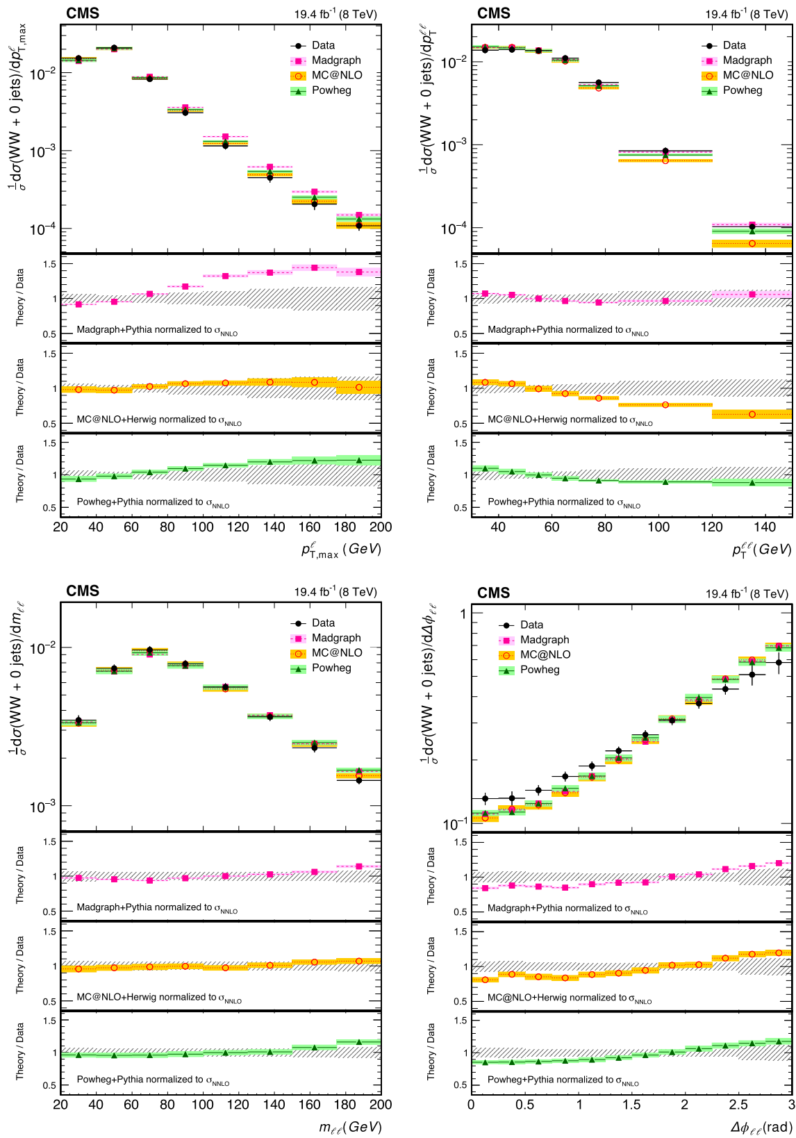
Fig. 3 Normalized differential W^+W^- cross section as a function of the leading lepton p_T ( p_{T,max}^\ell ) (top left), the transverse momentum of the dilepton system ( p_T^{\ell\ell} ) (top right), the invariant mass ( m_{\ell\ell} ) (bottom left) and the angular separation between leptons ( \Delta\phi_{\ell\ell} ) (bottom right).
