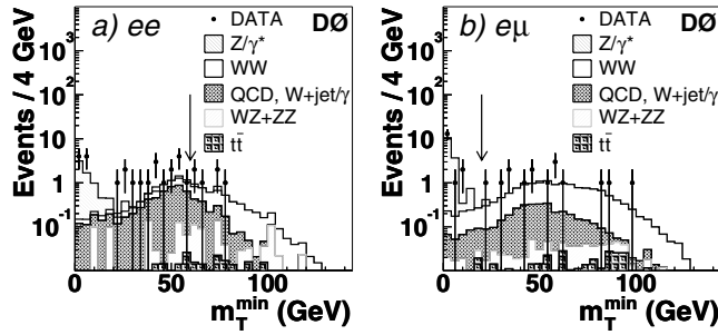
FIG. 2. Distribution of the minimal transverse mass m_T^{\min} after applying all selection criteria except the cut on m_T^{\min} for (a) the ee and (b) the e\mu channels. The arrows indicate the cut values.
