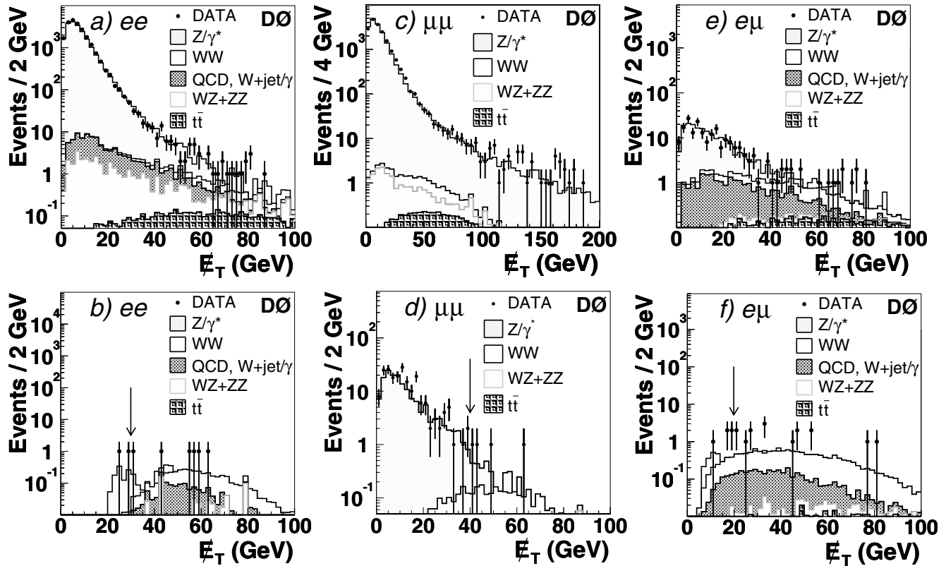
FIG. 1. Distribution of the missing transverse energy \cancel{E}_T after applying the initial transverse momentum cuts in the (a) ee , (c) \mu\mu , and (e) e\mu channel. Figures (b), (d), and (f) show the \cancel{E}_T distributions after the final selection except for the \cancel{E}_T criterion for the ee , \mu\mu , and e\mu channels, respectively. The arrows indicate the cut values. The QCD contribution is negligible in (c) and (d).
