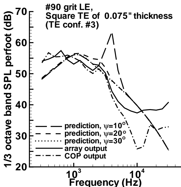
Figure 15. TE noise spectra predicted using measured boundary layer thickness and displacement thickness. Comparison to measured TE noise spectra. M=0.17 and airfoil is at -1.2 angle of attack. #90 grit on LE, with TE configurations #3 and 5.
