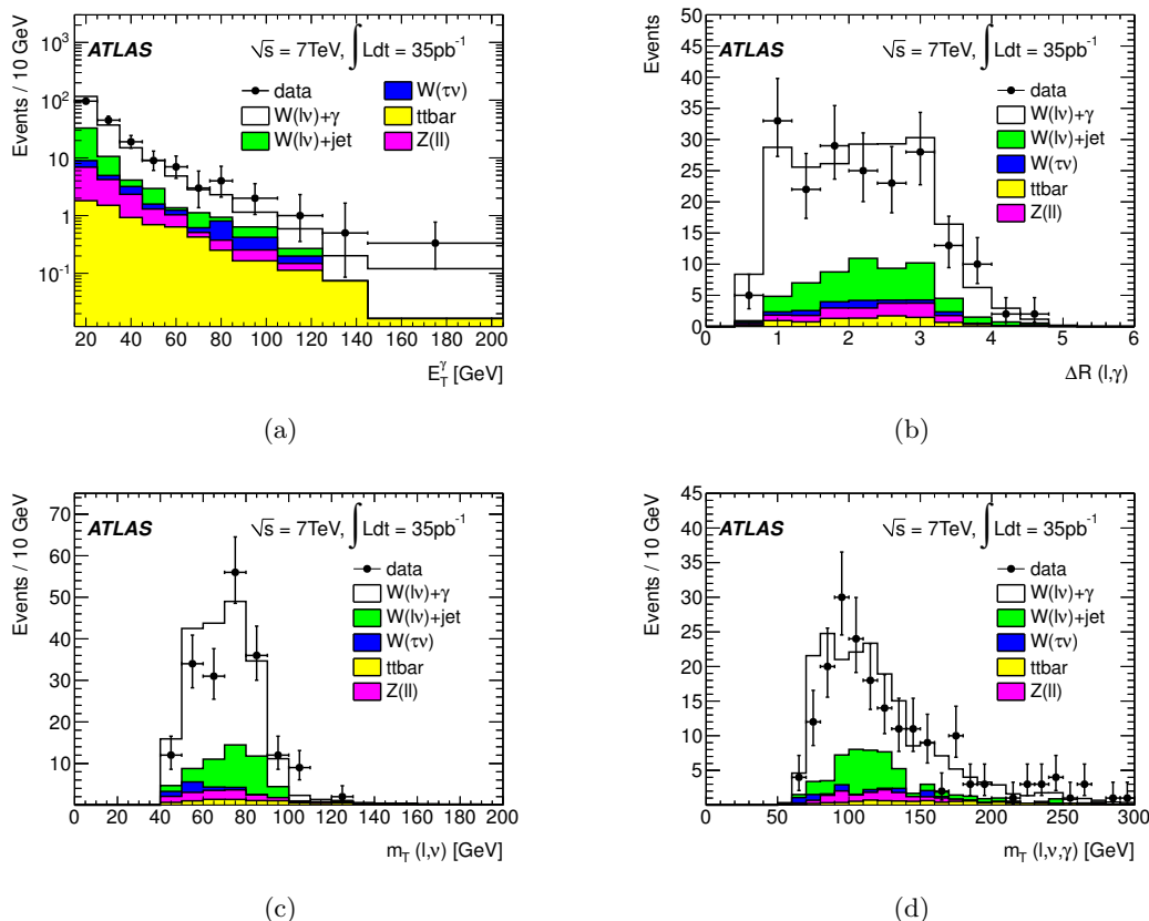
Figure 3. Distributions for the combined electron and muon decay channels of the photon transverse energy (a), \Delta R between lepton and photon (b), two body transverse mass ( m_T(l,\nu) ) (c) and three body transverse mass ( m_T(l,\nu,\gamma) ) (d) of the W\gamma candidate events. MC predictions for signal and backgrounds are also shown.
