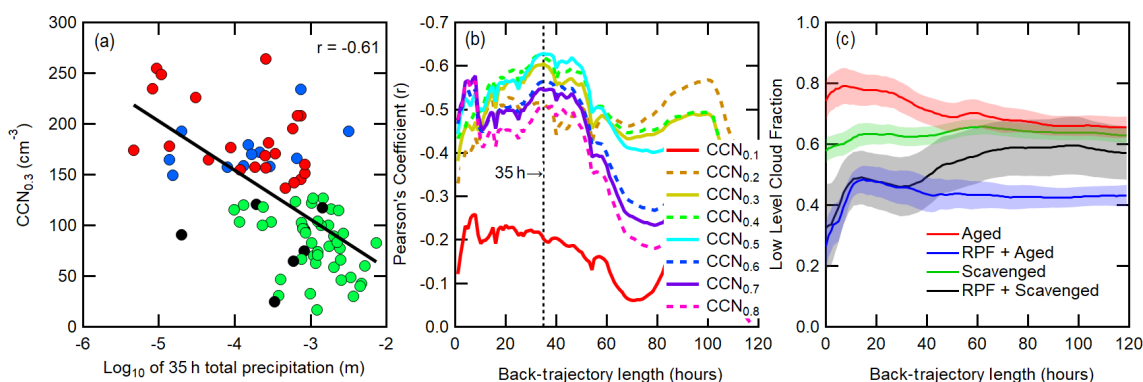
Figure 5. (a) Correlation of MBL CCN_{0.3} and total precipitation that occurred along a 35 h HYSPLIT back trajectory. Colors correspond to the legend in (c). (b) CCN and back-trajectory total precipitation correlation coefficient as a function of back-trajectory length. The vertical dashed line indicates a peak in correlation with CCN_{0.3} at 35 h. (c) Particle regime averaged ERA5 low-level cloud fraction over the 5 d back trajectory. Shaded areas represent the standard error.
