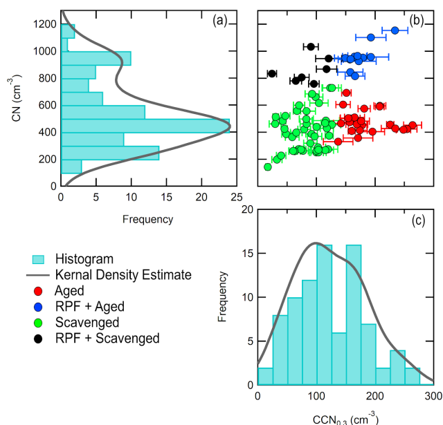
Figure 2. Histograms and kernel density estimates of (a) CN concentrations and (c) MBL CCN_{0.3} ( CCN concentration at 0.3 % supersaturation). (b) MBL CN and CCN_{0.3} . Measurements are divided into four particle regimes based on the observed bimodal distributions of both CN and CCN_{0.3} . Error bars represent the standard error.
