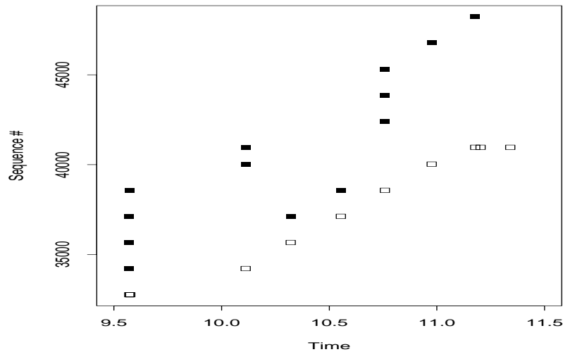
Figure 11.10: Solaris 2.4 retransmitting without cutting cwnd
