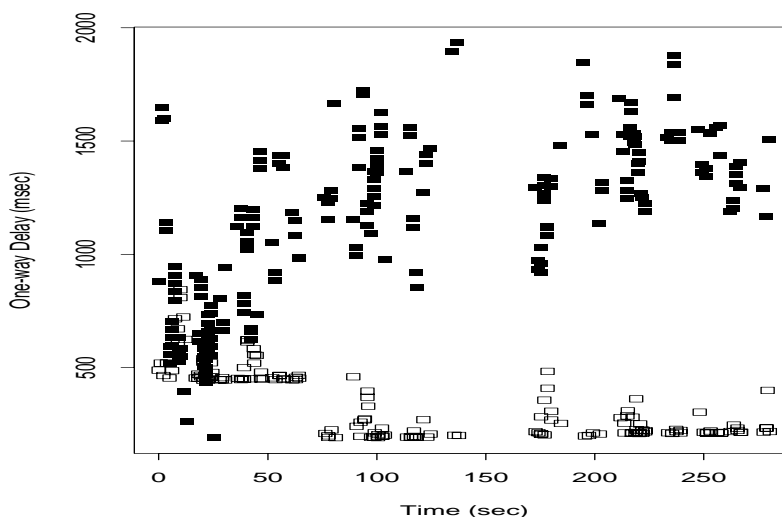
Figure 12.16: Clock adjustment masked by excessive network delays
