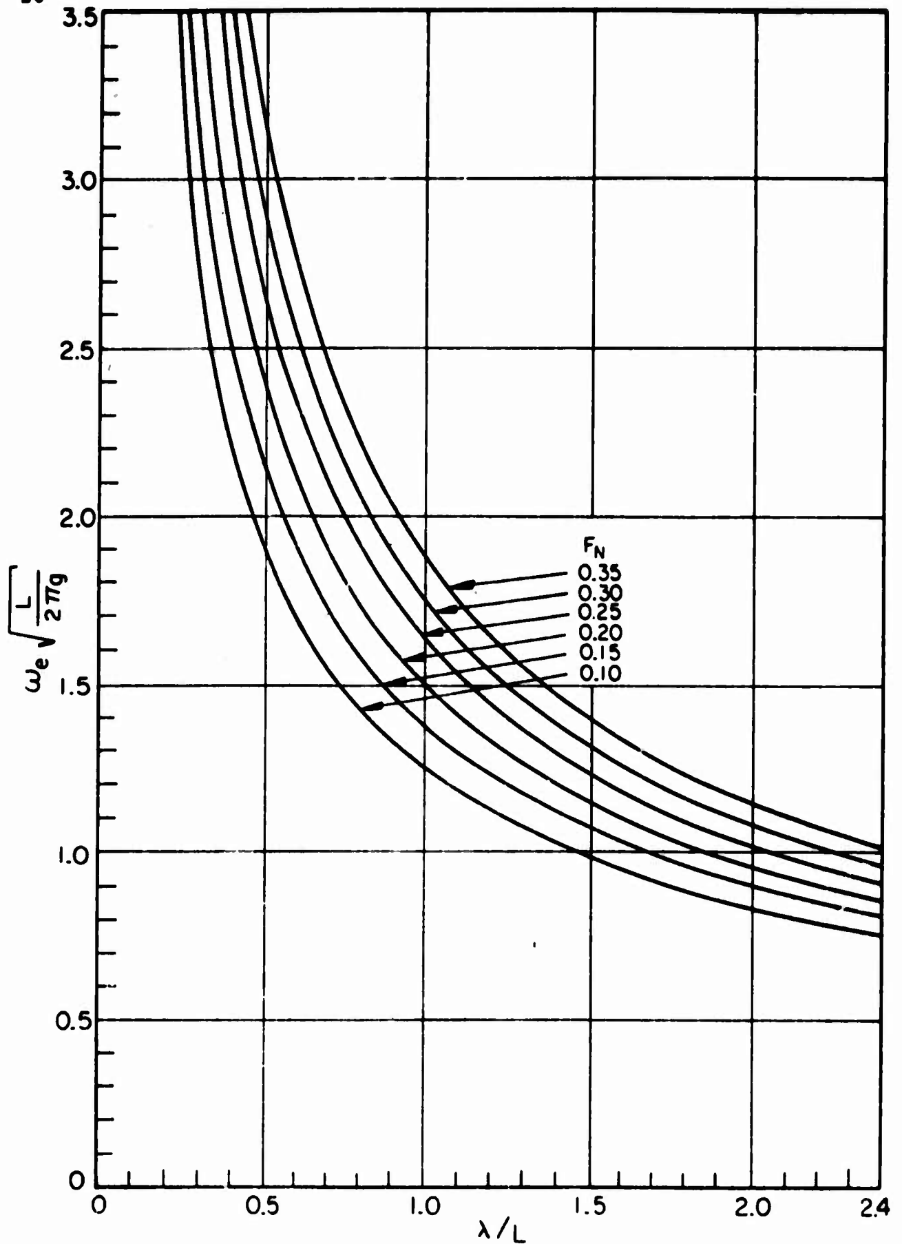
FIG. 9 RELATIONSHIP BETWEEN THE PERIOD OF ENCOUNTER AND THE WAVE LENGTHS FOR VARIOUS SHIP SPEEDS
