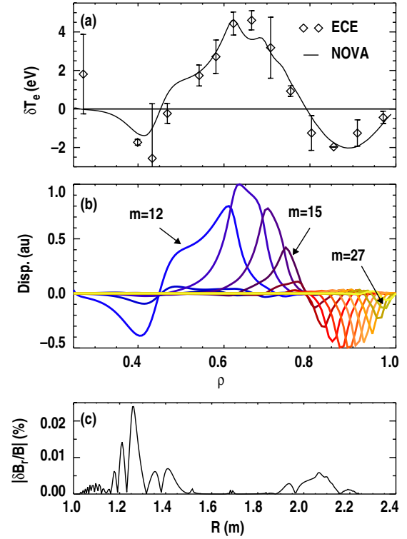
Figure 3. (a) Synthetic ECE diagnostic prediction (solid) using NOVA calculated f = 78 kHz global TAE from figure 2 overlaid with ECE measurements (diamonds). NOVA prediction scaled by single constant to match ECE data. (b) Poloidal harmonics comprising TAE from panel (a). (c) Calculated radial component of magnetic field fluctuation along device midplane (versus major radius) using amplitude obtained from comparison with ECE data.
