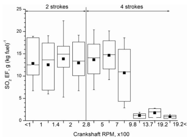
Fig. 10. SO 2 EF distribution among crankshaft rpm of the engine. The crankshaft range was divided into 11 bins based on logarithmic scale. Average SO 2 EFs of the bins are plotted along the y-axis, while sticks on the x-axis refer the borders of the bins.
