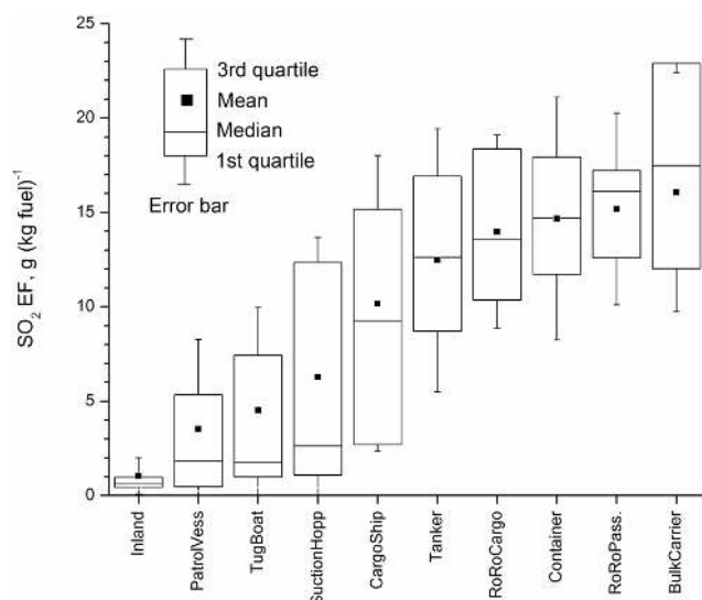
Fig. 9. SO 2 EF distribution among duty type of the ships.
