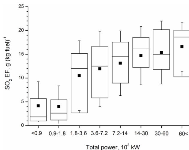
Fig. 11. The SO 2 EF distribution with the engine power of the ships. The power range of the ships was divided into 8 intervals based on logarithmic scale. Average SO 2 EFs of the bins are plotted along the y-axis, while power bins are marked on the x-axis.
