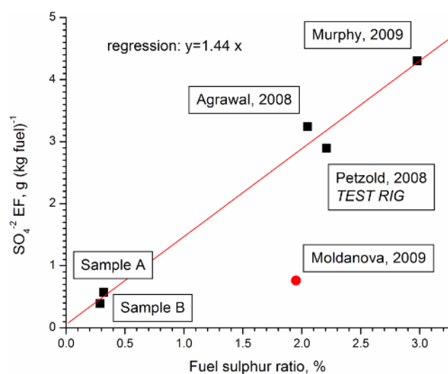
Fig. 14. The SO 4 2- EF as a function of fuel sulphur ratio. Red dot marks an outlier that was ignored during the regression calculation. Slope of the regression line: 1.44 \pm 0.1 , intercept forced to be zero, R^2 : 0.98.
