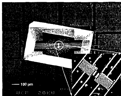
Figure 1. A scanning electron microscopy (SEM) image of the suspended heater structure. The lower insert is a higher magnification image of the two suspended membranes. The scale bar in the insert represents 10 \mu\text{m} .
