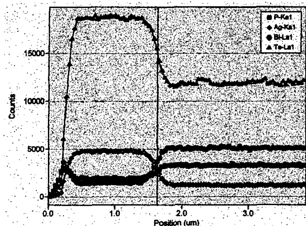
Figure 6. Energy dispersive X-ray spectroscopy (EDX) results starting from the bottom of a \text{Bi}_2\text{Te}_3 nanowire.
