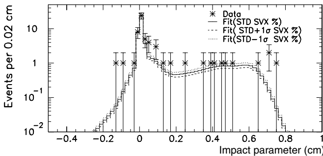
FIG. 19. The signed impact parameter distribution for conversions found in data. Solid line: Monte Carlo fit using the central value of f_{\text{conv}}^{\text{Good SVX}} . Dashed line: Monte Carlo fit increasing by one sigma. Dotted line: Monte Carlo fit decreasing by one sigma.
